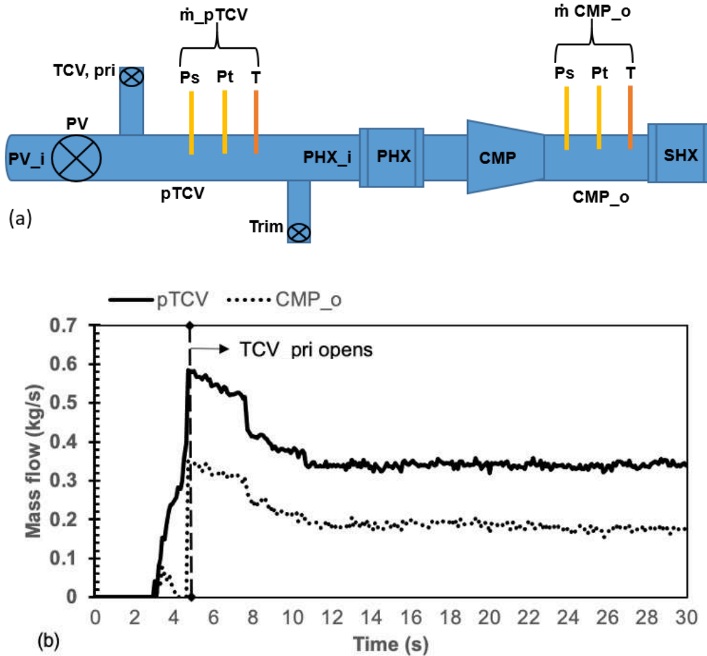
Figure 9: (a) Simplified schematic for mass flow measurements, (b) Measured mass flow as a function of test time at pTCV and CMP_o stations, 0 = PACK off.
