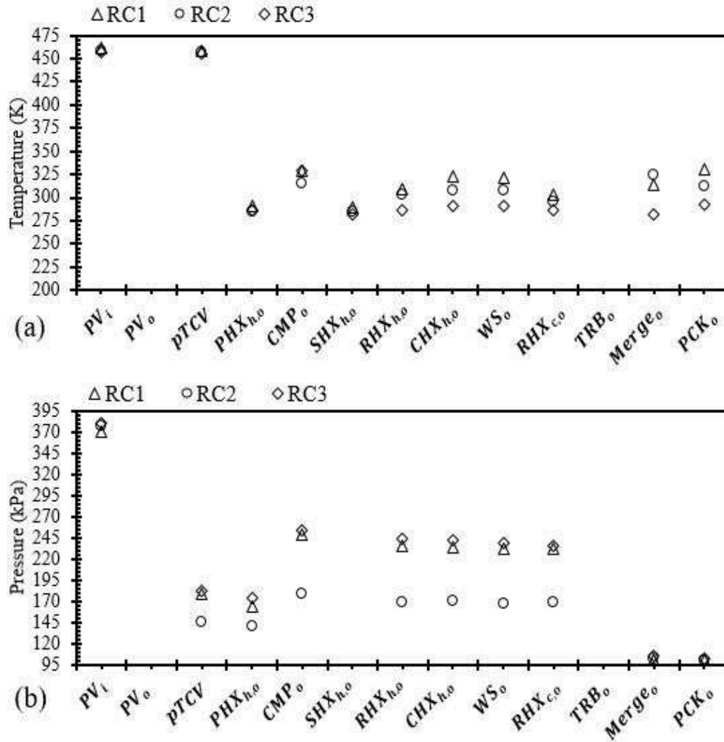
Figure 8 GTF repeatability test data, (a) Temperature, (b) Pressure.
