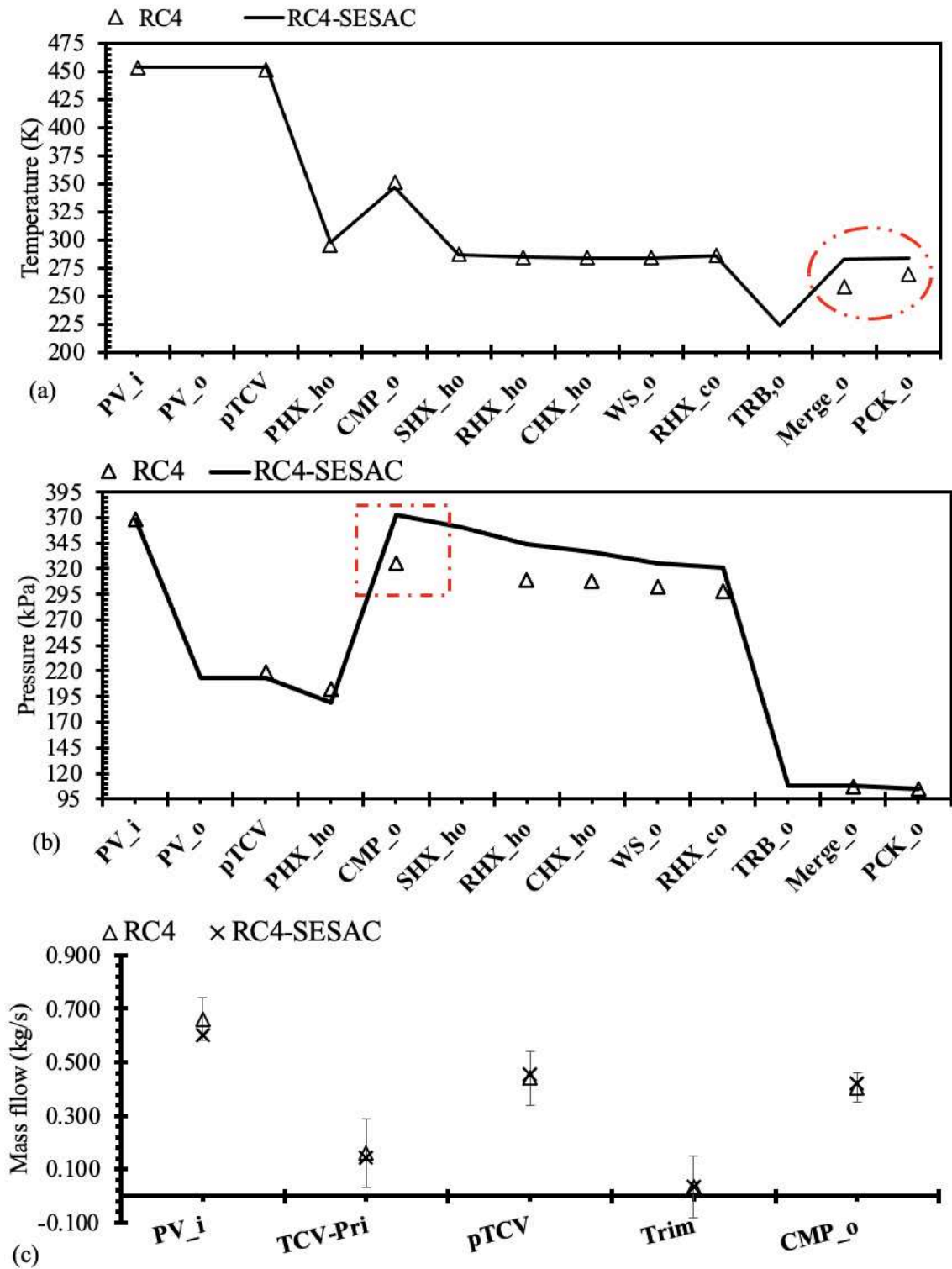
Figure 16 (a) Temperature profile, (b) Pressure profile and (c) Mass flow for RC4
