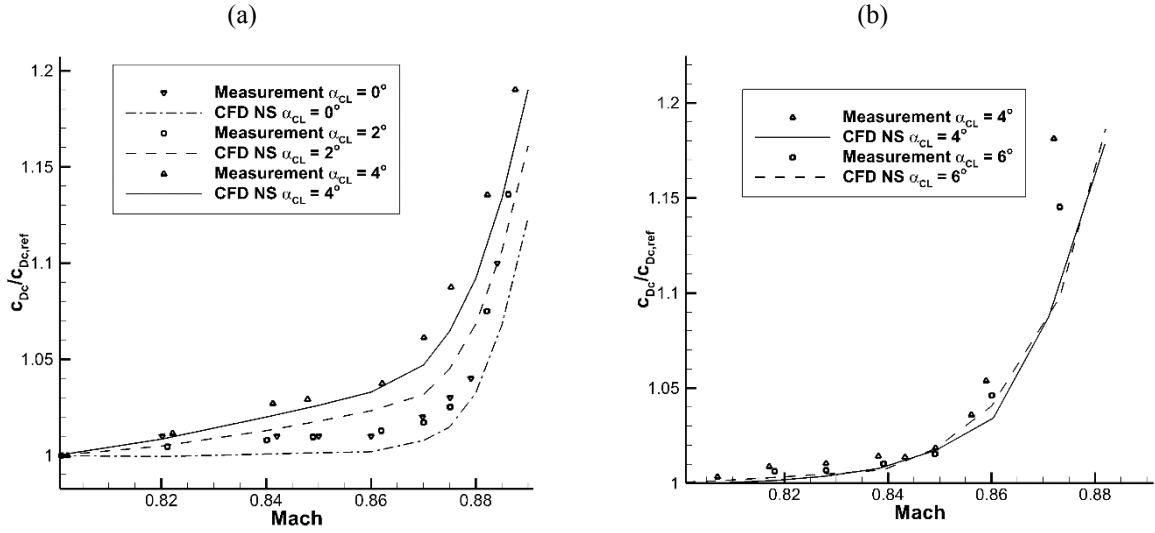
Figure 8 Effect of incidence on drag rise, normalised against drag at M=0.8 for (a) nacelle 2 at MFCR=0.7 and (b) nacelle 3 at MFCR=0.75
