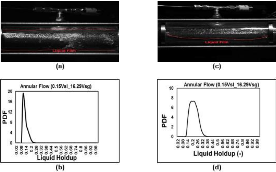
485 486 Figure 7: Typical annular flow regime ( V_{sl} = 0.15 m/s; V_{sg} = 16.29 m/s) in (a) concentric annulus, (b) PDF trend for concentric annulus (c) 487 fully eccentric annulus (d) PDF trend for fully eccentric annulus
