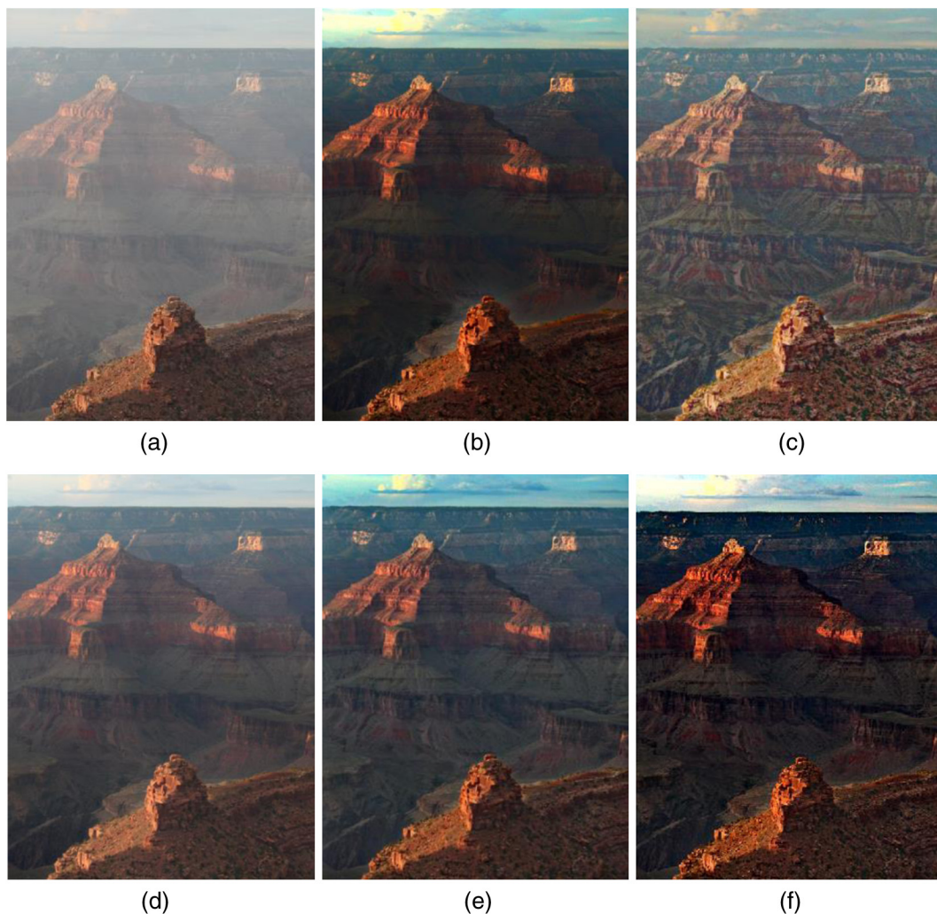
Fig. 2 The dehazed results: (a) the input hazy image 1, (b) result by DCP 8 with FOM3.42, (c) result by AVM 7 with FOM4.78, (d) result by CAP 14 with FOM3.93, (e) result by BCR 13 result with FOM3.93, and (f) the result of the proposed method with FOM5.19.
