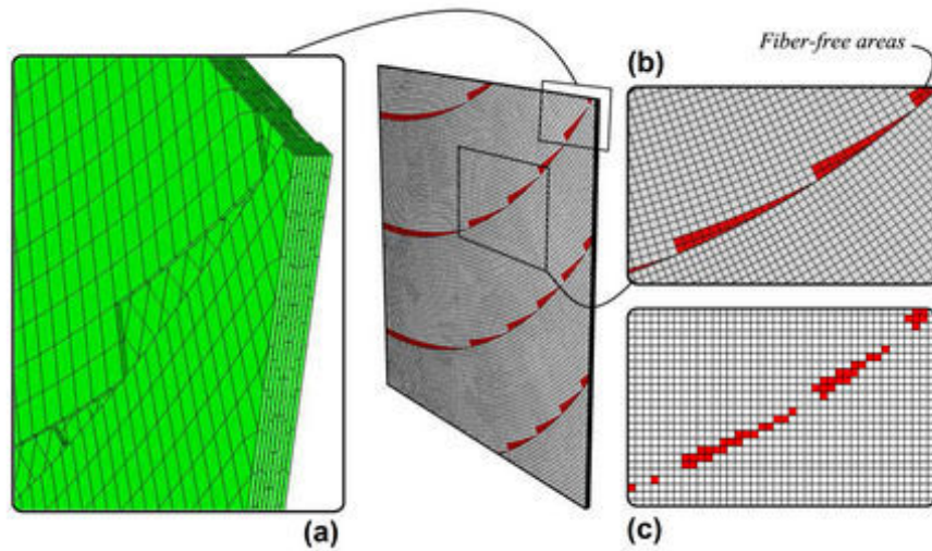
Figure 18: Finite element mesh generation of a VAT laminate; a) : Non-conforming mesh, b) : Tow-drop modeling of the fiber-free zones with structured mesh approach, c) : fiber-free zones in a regular mesh domain. Reproduced with permission from Falco et al. [63].
