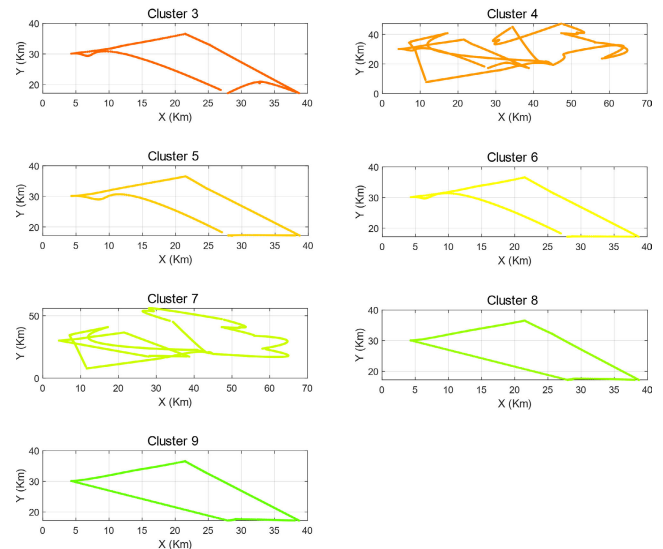
FIGURE 20. Scenario-3 DBSCAN detected mission cluster plots.
