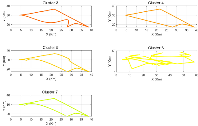
FIGURE 16. Scenario-2 DBSCAN detected mission cluster plots.
