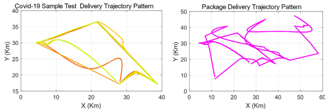
FIGURE 17. Scenario-2-detected combined mission patterns.
