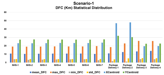
FIGURE 28. Scenario-1: NHS and DS missions DFC statistical distribution.
