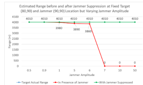
Figure 13 Estimated range for a Fixed Target and Jammer with varying strength
