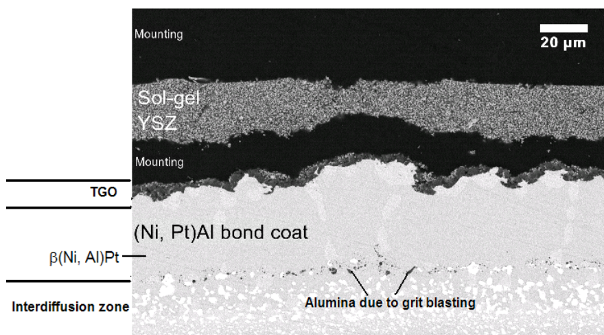
Fig. 8 : Cross section (SEM) of the (YSZ SG/ (Ni, Pt)Al/ AM1) sample after 200 cycles of 1 hour at 1100°C.
