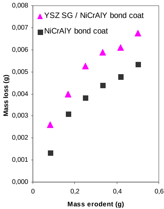
Fig. 3 : Mass loss of the YSZ SG top coat deposited on the NiCrAlY bond coat versus the mass of the erodent projected at their surface.
