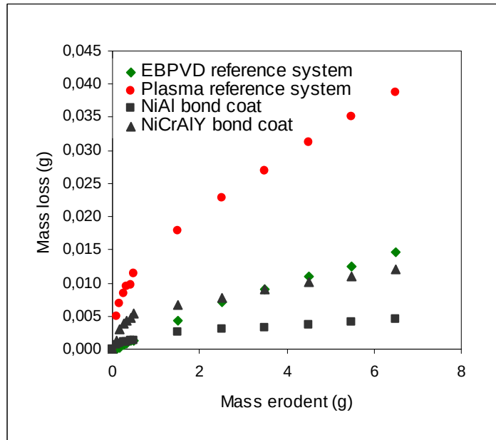
Fig. 2 : Mass loss of the reference samples versus the mass of the erodent projected at their surface.
