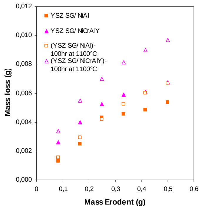
Fig. 5 : Mass loss of the aged 100hr at 1100°C and not aged YSZ SG samples versus the mass of the erodent projected at their surface.
