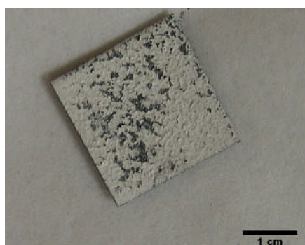
Fig. 9 : Photograph of the surface of the system (YSZ SG/ NiCrAlY/ Hastelloy X) after 740 cycles of 1 hour at 1100°C.
