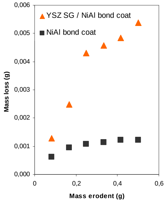
Fig. 4 : Mass loss of the YSZ SG top coat deposited on the NiAl bond coat versus the mass of the erodent projected at their surface.
