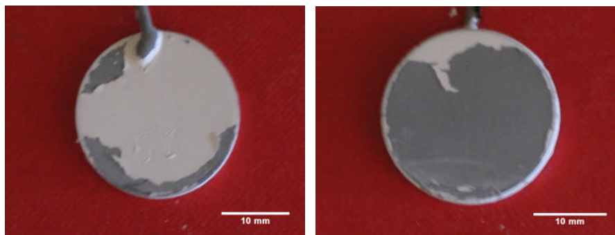
Fig. 7 : Images of (YSZ SG/ (Ni, Pt)Al/ AM1) sample after 200 cycles of 1 hour at 1100°C (recto : left ; verso : right).
