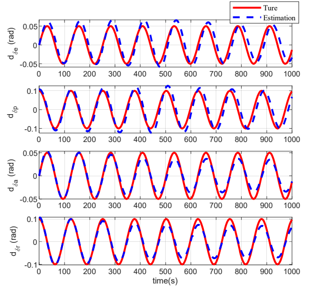
Fig.7 Unknown observable disturbance estimation without control allocation
