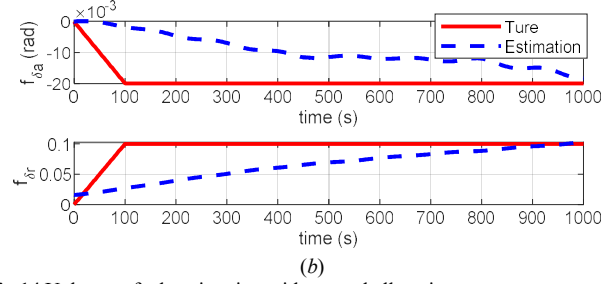
Fig.14 Unknown fault estimation with control allocation
