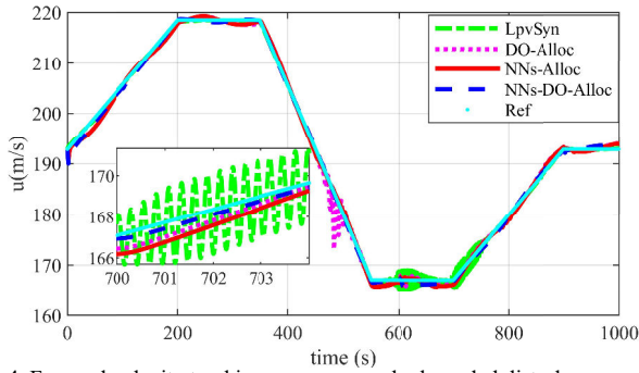
Fig.4. Forward velocity tracking responses under bounded disturbances
