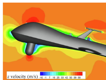
Fig. 11 Stream-wise velocity contours at symmetry plane of MQ-1 UCAV showing recirculation zones behind external geometrical modifications.
