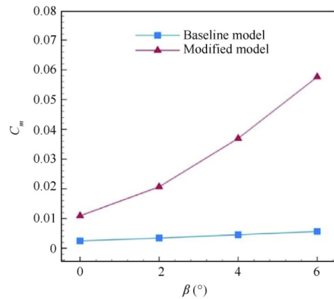
(b) Angle of bank \beta
