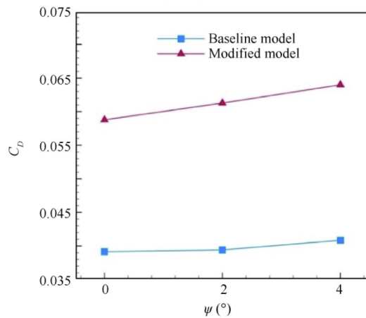
(c) Angle of yaw \psi
