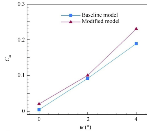
(c) Angle of yaw \psi
