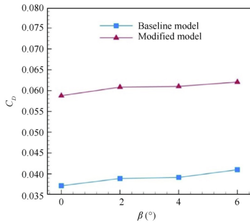
(b) Angle of bank \beta
