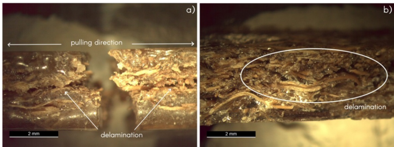
Fig. 15. Fracture section from a 60% w/w ATF/PLA biocomposites showing delamination after failure at the tensile test.
