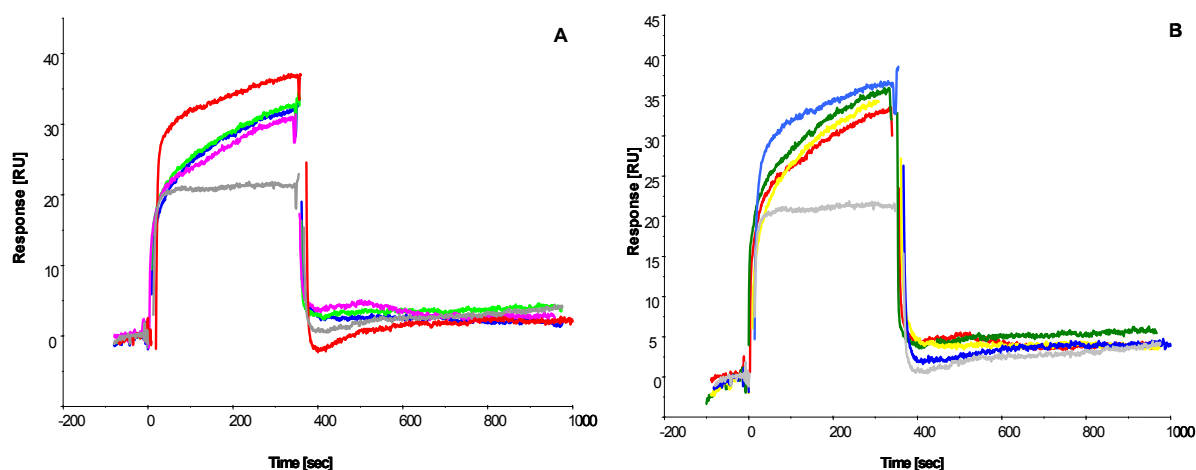
Figure 5. Sensorgrams showing the binding interaction of immobilized (A) octamer peptide CSIVEDGL and (B) 13-mer peptide GPAGIDGPAGIRC with decreasing ochratoxin A-BSA analyte concentration (from top to bottom: 100, 1, 0.1, 0.01 mg L -1 ; equivalent to 15pM–0.15 μM. BSA reference binding is shown in grey).
