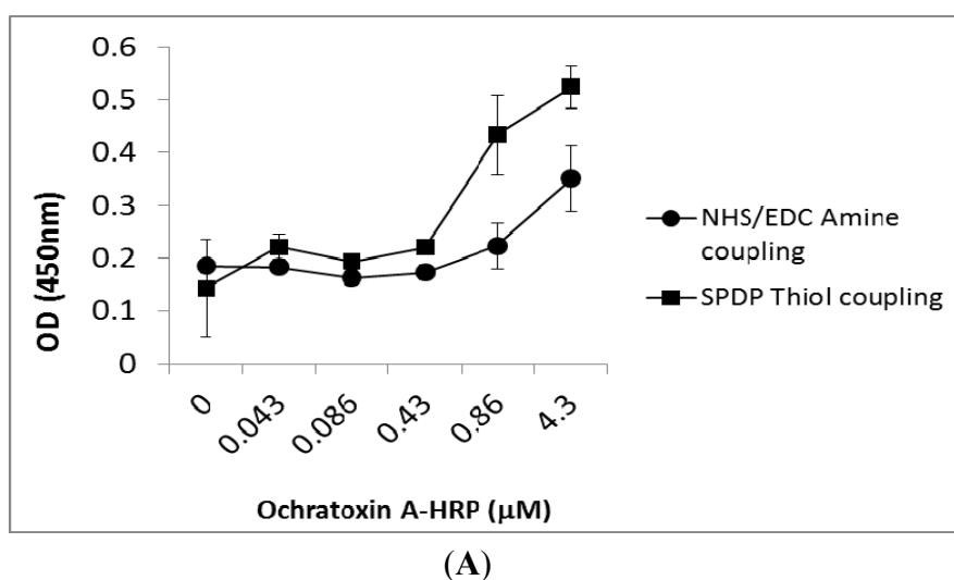
Figure 3. Capacity of the ochratoxin A-HRP to bind to the octapeptide and 13-mer peptide. The interaction between serial dilutions of HRP-conjugated ochratoxin A and octapeptide (A) and 13-mer peptide (B) immobilized to functionalized microtitre plates via amine coupling (●) and thiol coupling (■) is expressed as absorbance at A 450 nm versus ochratoxin A-HRP concentration ( \mu M). Error bars illustrate the mean and standard deviation of multiple experiments.
