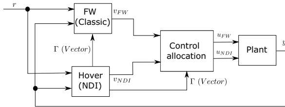
Fig. 2. Unified VSTOL control scheme schematic.
