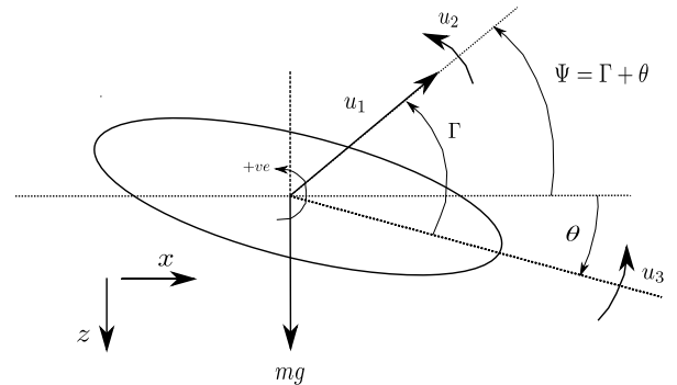
Fig. 1. PVTOL hover schematic.
