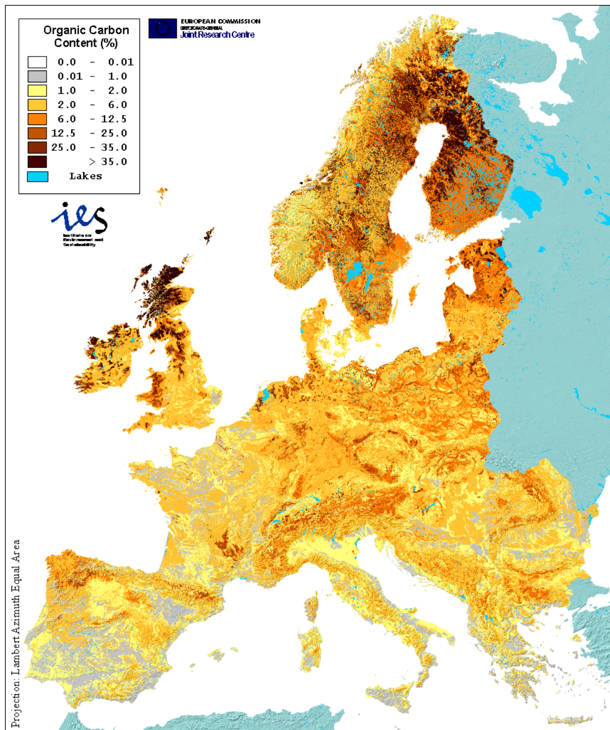
Figure 1. Organic carbon content (%) in topsoils (0–30cm) in Europe (adapted from Jones et al. , 2004).
