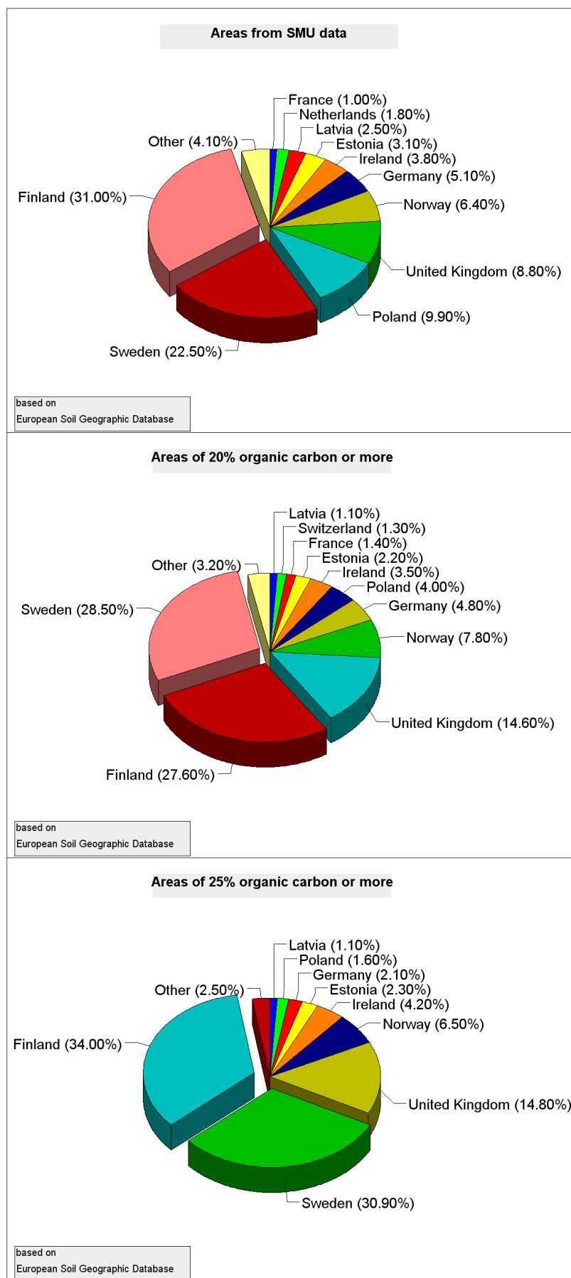
Figure 4: Distribution of peat and peat topped soils (0–30cm) in Europe, based on: (a) European Soil Database v 1.0; (b) Map of OC in Topsoils of Europe , with threshold of OC \geq 20\% ; and (c) Map of OC in Topsoils of Europe , with threshold of OC \geq 25\% .
