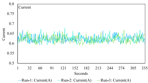
FIGURE 11. Current measurements for R1, R2, and R3.
