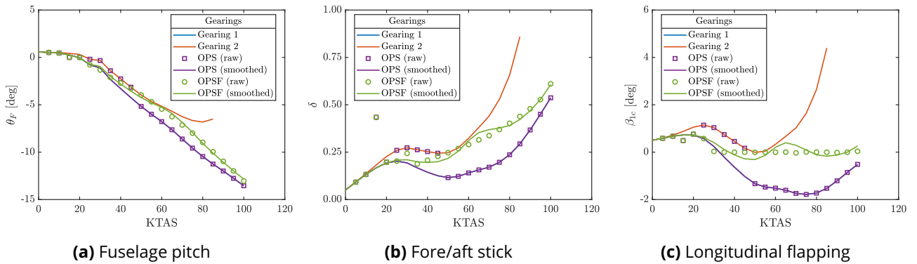
Figure 4: Trim parameters at 0° rotor tilt angle.
