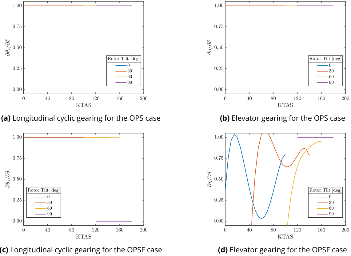
Figure 3: Smoothed optimisation data for the OPS and OPSF cases.
