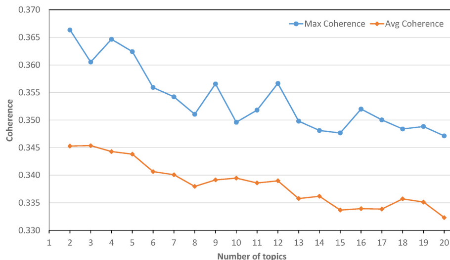
Fig. 6. Maximum and average coherence per topic configuration.
