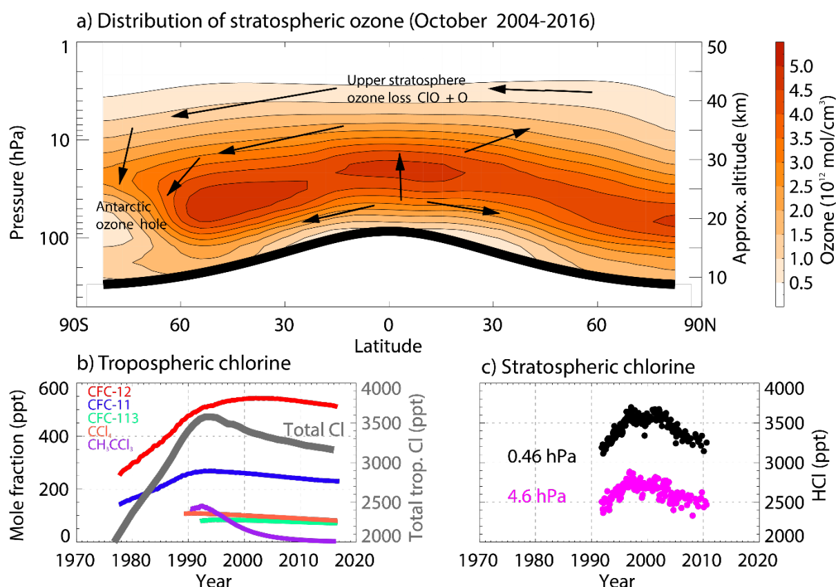
Figure 1. Latitude-height cross section of stratospheric ozone and time series of chlorine in the troposphere and stratosphere. (a) October mean (2004-2016) ozone concentration (10 12 molecules/cm 3 ) from the Microwave Limb Sounder (MLS) instrument aboard the Aura satellite 89 . The thick black lines denotes the location of the climatological tropopause 90 . Annotated text shows the main regions where ozone is most severely destroyed by halogens. The black arrows indicate the Brewer-Dobson circulation which transports air upwards in the tropics, polewards and downwards at high latitudes, with stronger transport towards the winter pole. (b) Observed monthly mean surface mole fraction (ppt) of selected ozone-depleting substances (left axis, see legend for colour coding) from the National Oceanic and Atmospheric Administration (NOAA) long-term monitoring program 91 . The thick grey line shows the evolution of total tropospheric chlorine (includes contributions from other halocarbons, e.g. HCFCs) from the World Meteorological Organization A1 scenario (right axis). (c) Time series of monthly mean HCl (ppt) in the tropical upper stratosphere (4.6 hPa, ~40km, pink) and lower mesosphere (0.46 hPa, ~55km, black) from the GOZCARDS satellite measurement compilation 46 . HCl is a degradation product of chlorine-containing ODSs and increases with altitude.
