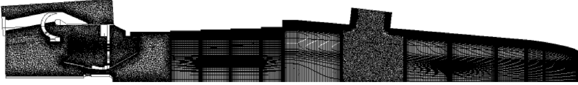
Fig. 3. Computational mesh of the quarter-model [11].
