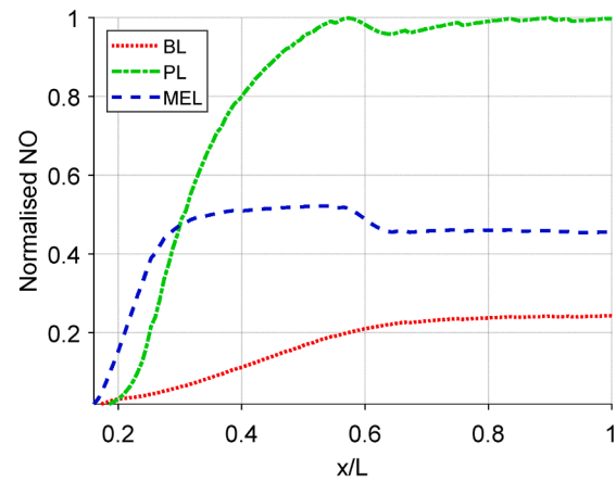
(b) Normalised NO (ref. to PL)
