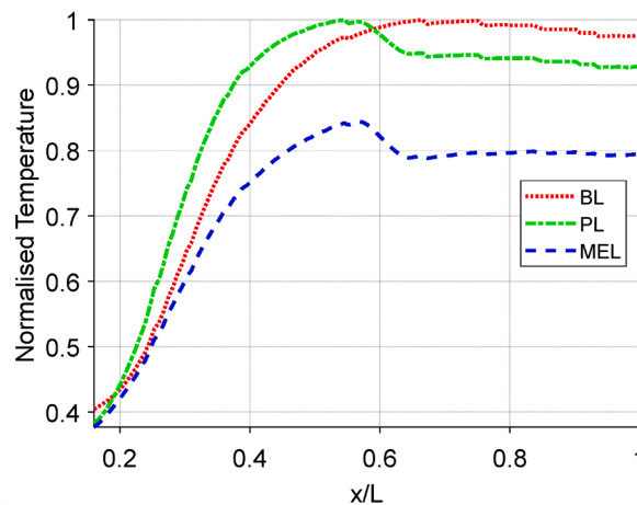
(c) Normalised Temperature (ref. to PL)
