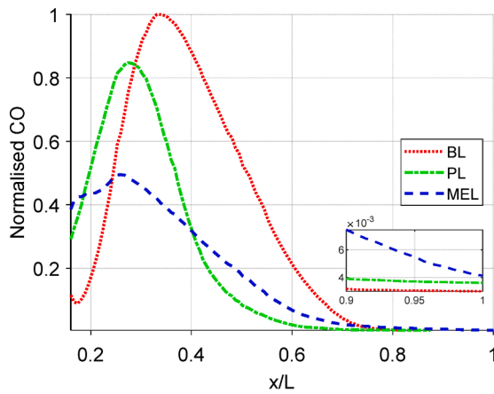
(a) Normalised CO (ref. to BL)
