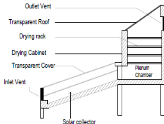
Fig. 8 Mixed-mode solar dryer with its sectional view [Source: Bolaji and Olalusi, (2008)].
