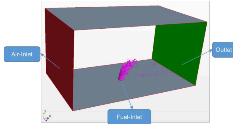
Figure 13 Schematic of the calculation domain
