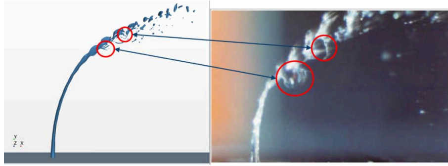
Figure 9 Comparison of the simulation result with experiment photo ( t = 3.83 ms)
