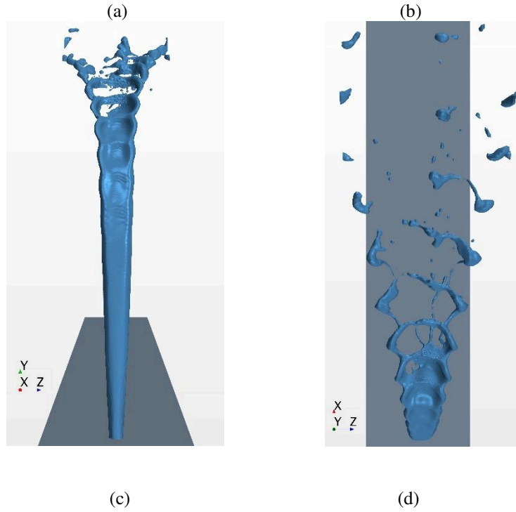
Figure 7 Various views of the boundaries of the liquid jet ( t = 3.83 ms)
