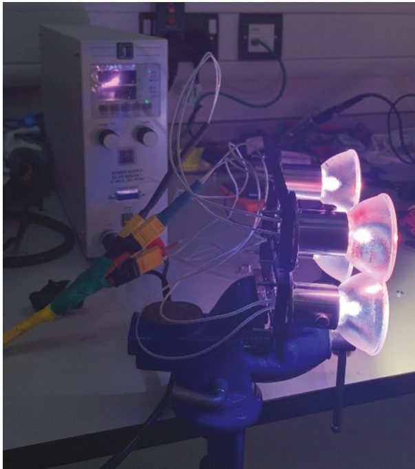
Figure 3. View of the halogen lamp array composed of four 250 W bulbs.
