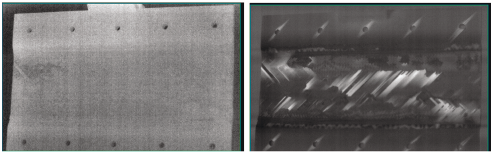
Figure 31. (A) A cold image of a damaged composite sample before excitation. (B) A thermal image of a post-processed image of a composite sample after excitation.
