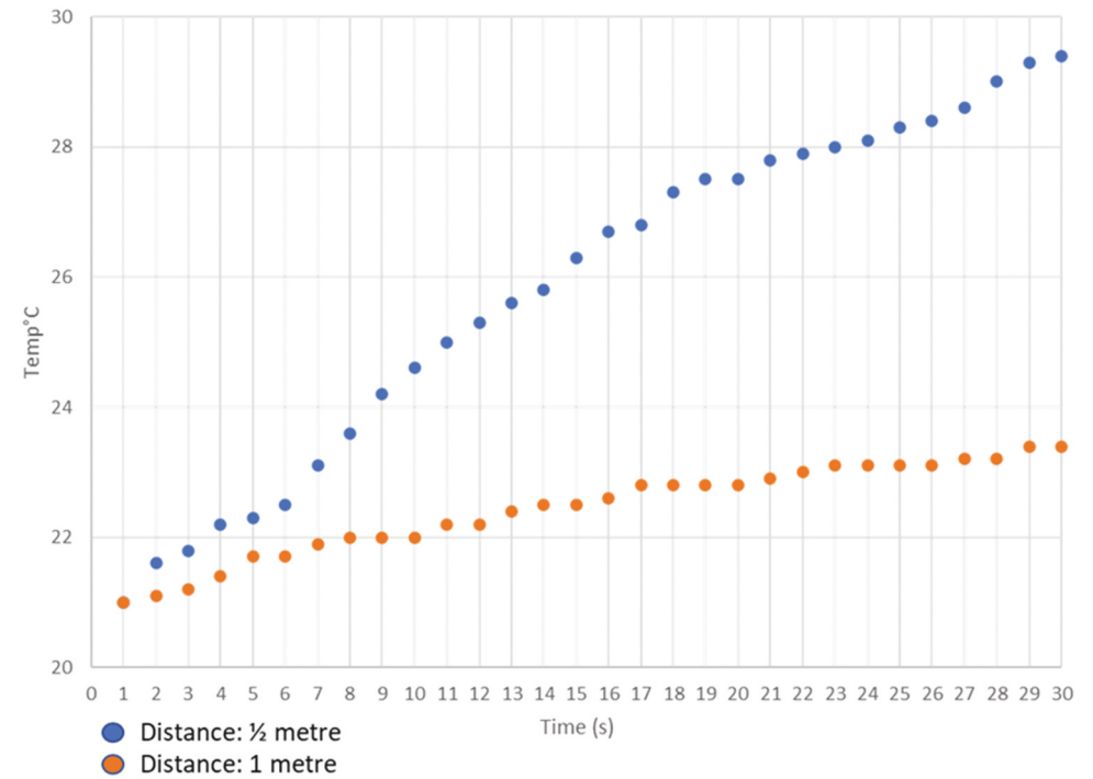
Figure 8. Surface temperature increase over time when heating a composite with the lamp assembly at both half a metre (blue dots) and one metre (Orange dots) from the sample.
