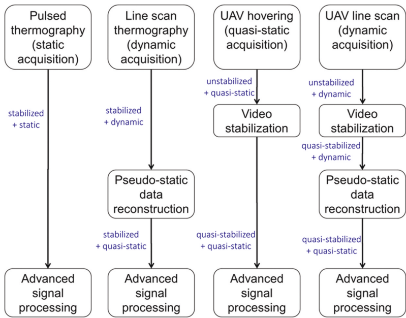
Figure 32. Dynamic and static thermography approaches.
