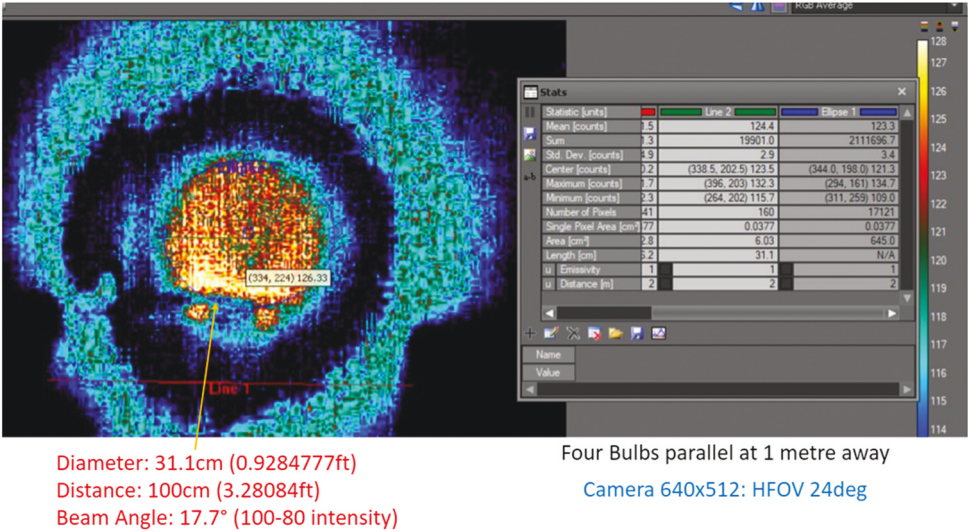
Figure 16. The image is a screenshot from the ResearchIR software showing an IR image taken of the bulbs exciting a surface. A line is drawn across the uniform excited surface and the details can be seen in the table within the image named 'Line 2'.
