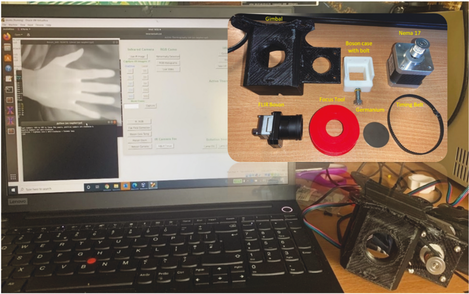
Figure 33. Developed focus mechanism for the FLIR Boson.
