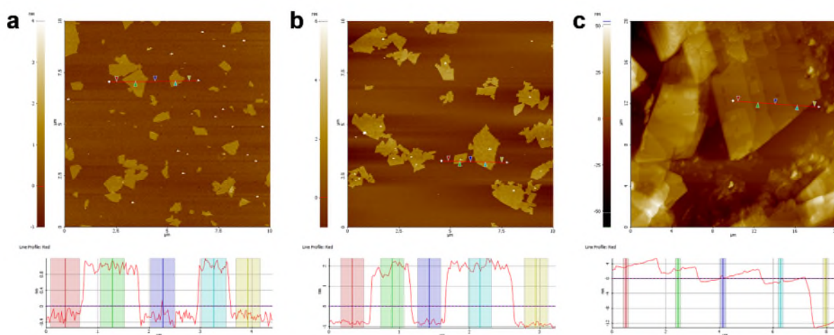
Figure 3. AFM images of (a) GO, (b) PC-rGO, and (c) AA-rGO deposited on Si/SiO 2 wafers surface.
