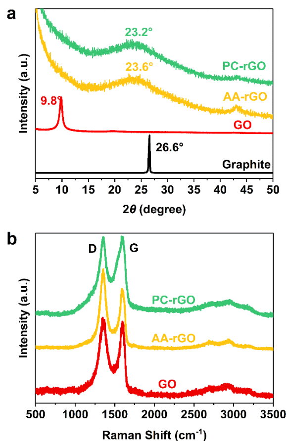
Figure 2. (a) XRD patterns of graphite, GO, AA-rGO and PC-rGO, and (b) Raman spectra of GO, AA-rGO and PC-rGO.
