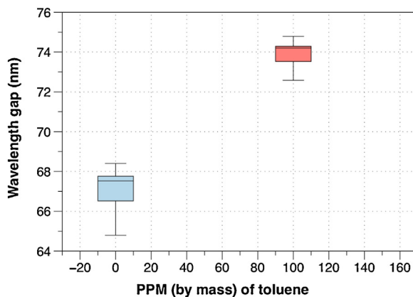
Fig. 8. Box and whisker plot of the sensor readings while immersed in water compared with immersion in 100 ppm toluene solution ( n=6 ).
