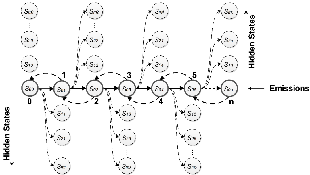
Fig. 2 A theoretical model for EDP sequencing [8]
