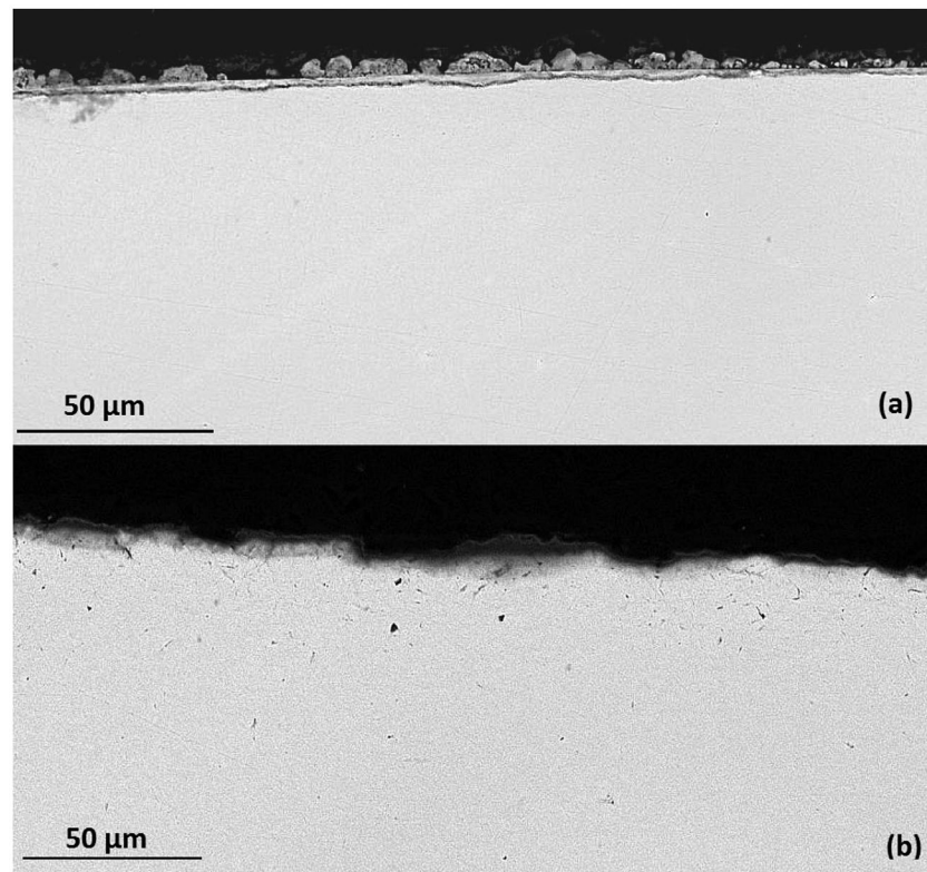
Figure 4. Unstressed corrosion product at 550 °C and exposed to 5 µg/cm 2 /h with a test gas of air – 300 vppm SO 2 (a) 500 h resulting in 7.7 µm oxide scale (b) 100 h exposure resulting in 2.43 µm oxide scale.
