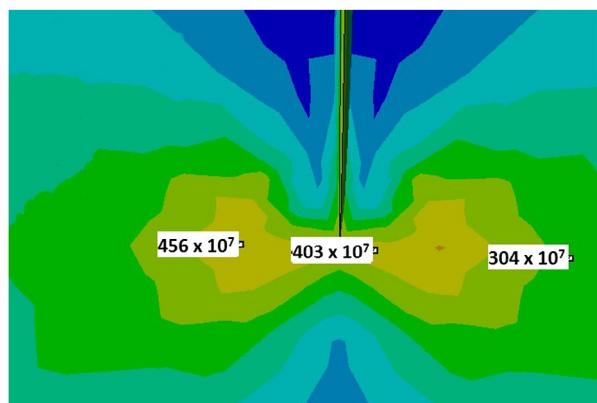
Figure 10. Stress distribution around a centrally located 100 µm crack tip in a C-ring at 890 MPa.
