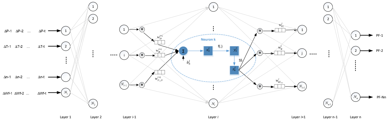
Fig. 1 1DCNN architecture.
