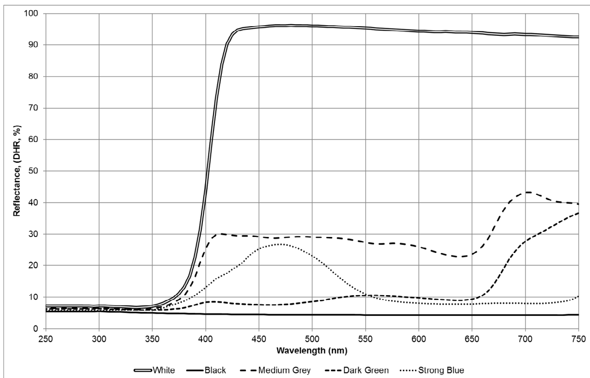
Figure 11 Some empirical \text{TiO}_2 based paint reflectivities for different wavelengths (visible colour differences shown)
