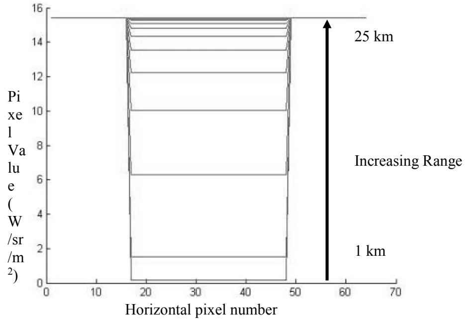
Figure 4 'Black' case showing contrast changing at various ranges
