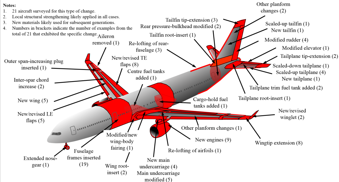
Figure 17: Design changes for both increasing range and payload.
