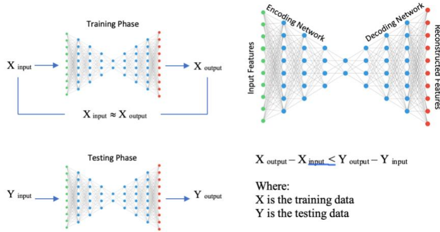
Fig. 2 Evaluating reconstruction errors with autoencoders
