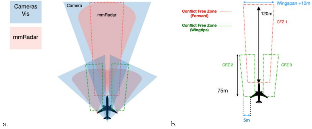
Fig. 3 Distribution of sensors (a) and conflict free zone dimensions (b)
