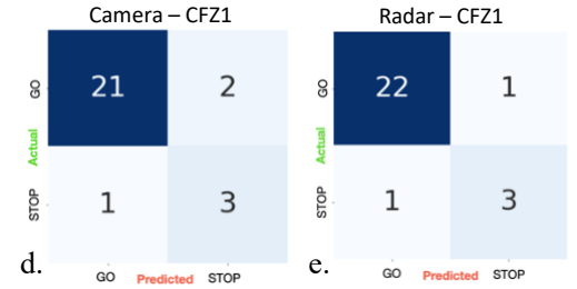
Confusion Matrices
