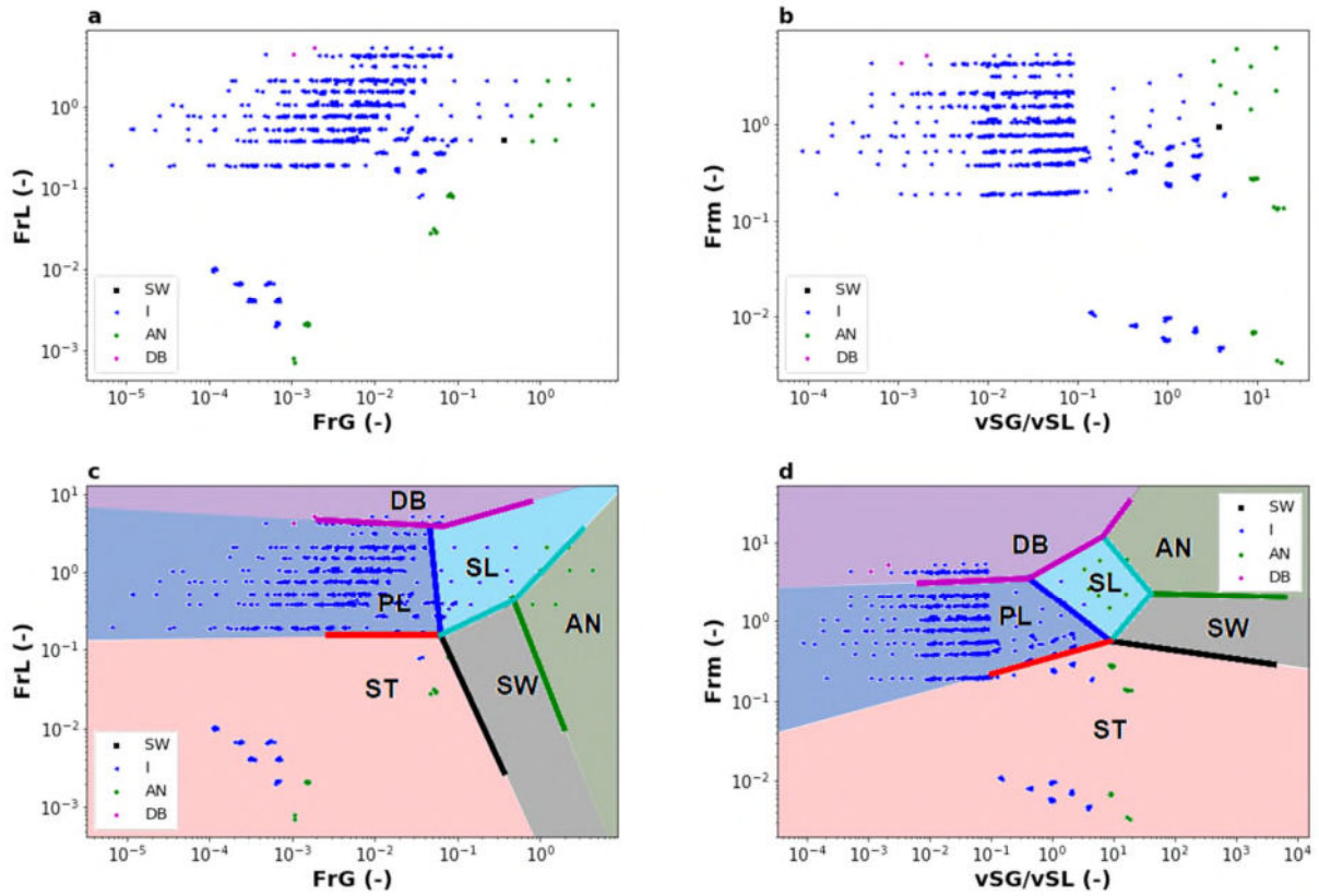
Fig. 5: Superimposing the transition boundaries of datasets extracted from experimental works in the literature on the datasets from MultiFlowMet II projects; (a) Fr_L versus Fr_G ; (b) Fr_m versus v_{SG}/v_{SL} . (c) Fr_L versus Fr_G with transition boundaries; (d) Fr_m versus v_{SG}/v_{SL} with transition boundaries.
