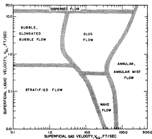
Fig. 1: Gas-liquid flow regime map in horizontal pipe (Mandhane et al., 1974).
