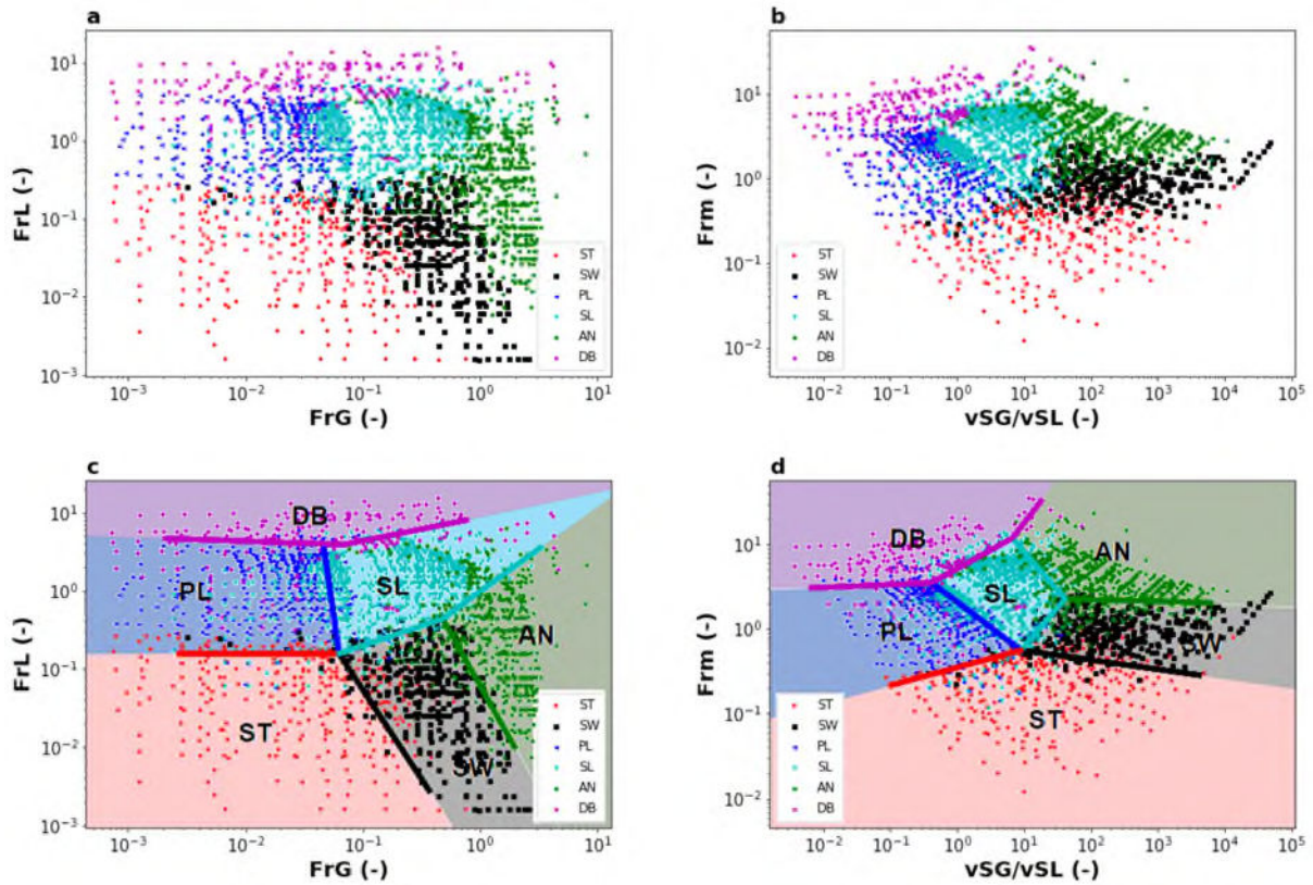
Fig. 3: Constructing transition boundaries for datasets extracted from experimental works in the literature; (a) Fr_L versus Fr_G ; (b) Fr_m versus v_{SG}/v_{SL} (c) Fr_L versus Fr_G with transition boundaries; (d) Fr_m versus v_{SG}/v_{SL} with transition boundaries.
