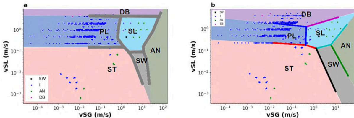
Fig. 4: The flow map of superficial liquid velocity ( v_{SL} ) versus superficial gas velocity ( v_{SG} ) based on the datasets from MultiFlowMet II projects, (a) superimposed Mandhane et al. (1974) flow map, (b) with constructed transition boundaries.
