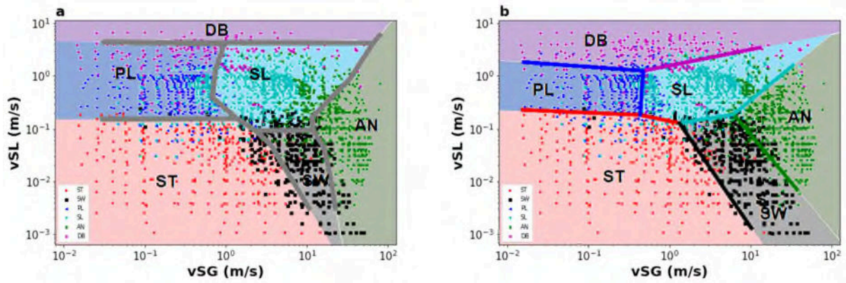
Fig. 2: The flow map of superficial liquid velocity ( v_{SL} ) versus superficial gas velocity ( v_{SG} ) based on gathered literature datasets, (a) with superimposed Mandhane et al. (1974) flow map, (b) with constructed transition boundaries.
