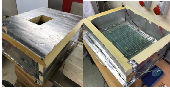
Figure 5 Celotex chamber
