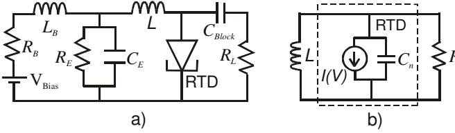
Figure 3: a) Typical single RTD oscillator schematic circuit diagram, b) RF equivalent circuit diagram of RTD oscillator, with the RTD modelled as voltage controlled current source and its self-capacitance, but with its contact resistance neglected.
