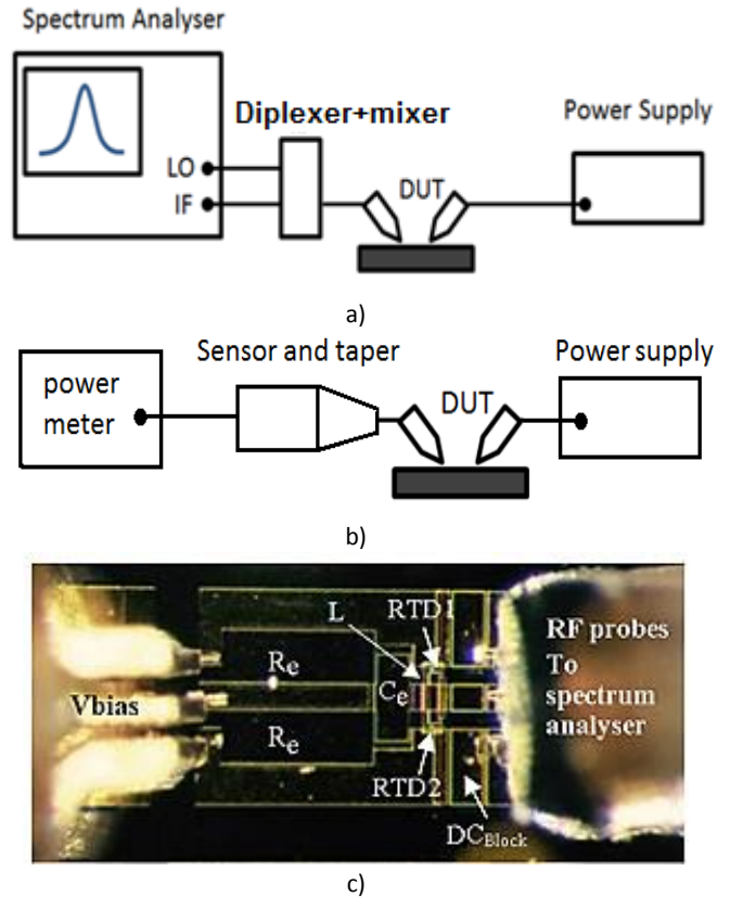
Figure 8: Schematic block diagram showing on-wafer measurements setup: (a) Spectrum measurement, (b) Power measurement, and (c) Micrograph of fabricated oscillator during on-wafer measurement.
