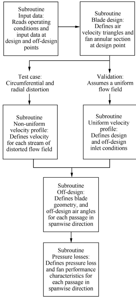
Fig. 2 Structure of fan performance program.
