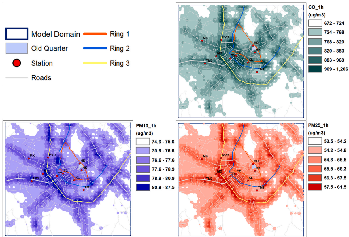
Fig. 3. Spatial maps of hourly mean modelled (a) CO, (b) PM 10 , and (c) PM 2.5 . © OpenStreetMap contributors 2020. Distributed under a Creative Commons BY-SA License.
