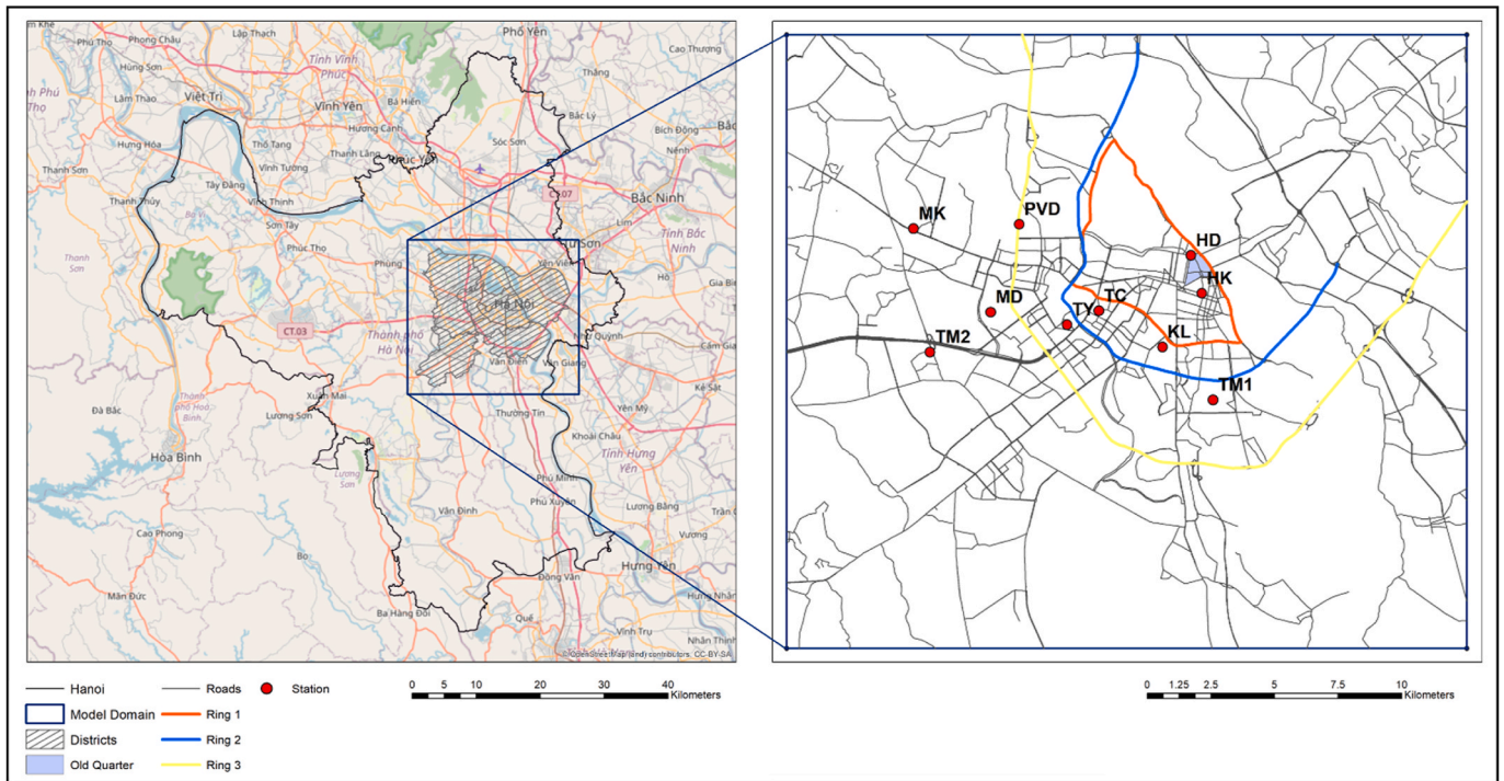
Fig. 2. Model domain and air quality monitoring stations in Hanoi. © OpenStreetMap contributors 2020. Distributed under a Creative Commons BY-SA License.
