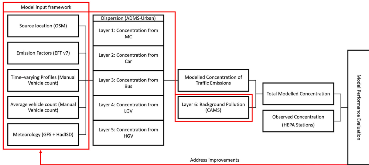
Fig. 1. Visual structure of this study's structure.
