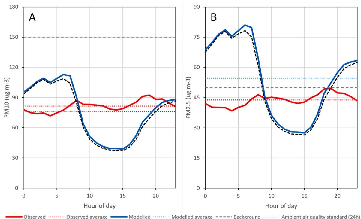
Fig. 5. Mean diurnal variation of modelled and observed (a) PM_{10} , and (b) PM_{2.5} concentrations.
