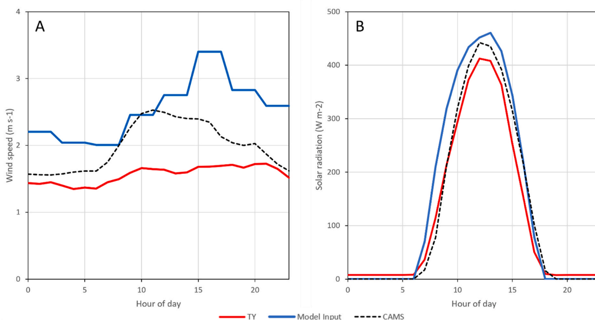
Fig. 6. Mean diurnal variation of (a) wind speed, and (b) solar radiation.
