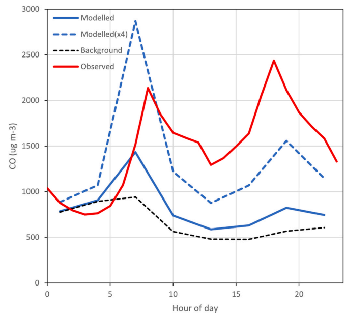
Fig. 4. Mean diurnal variation of modelled and observed CO concentrations. Modelled = modelled concentration of traffic emission + background. Modelled (x4) = 4x modelled concentration of traffic emission + background.
