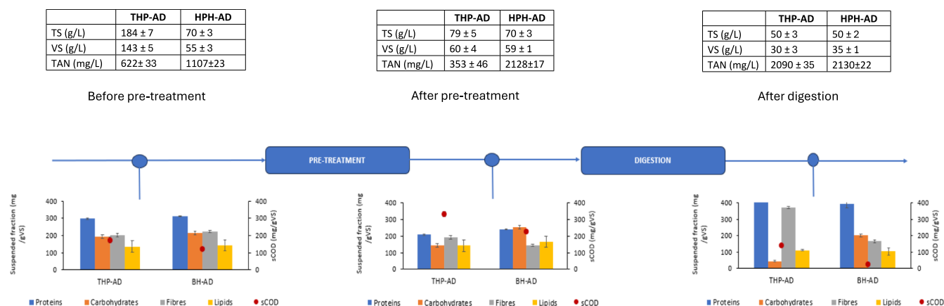
Fig. 1. Distribution of suspended macromolecules fractions and sCOD across the sludge treatment chain in the studied full-scale THP- and BH-AD sites indicated along with solids characterisation and TAN levels.
