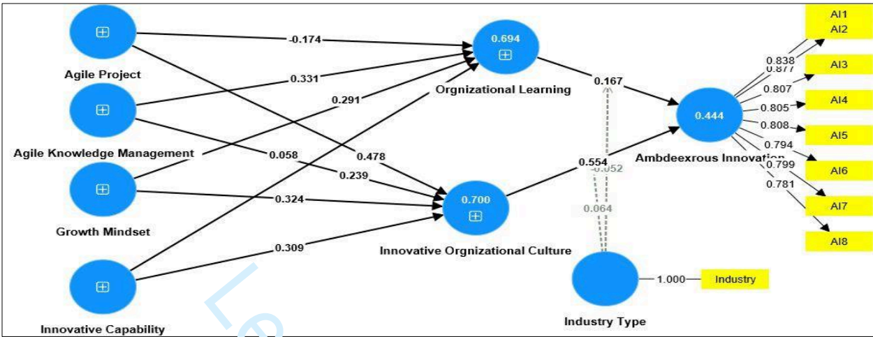
Figure 2: Measurement Model
