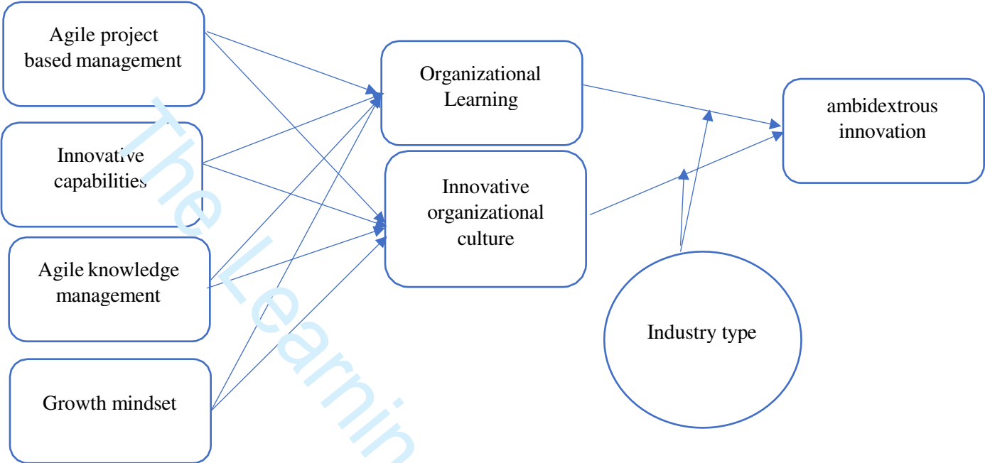
Figure 1: Conceptual Framework
