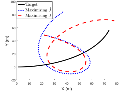
(c) Robot and target trajectories of case 3
