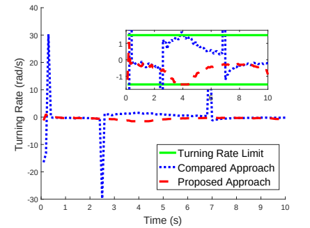
(c) Robot turning rate
