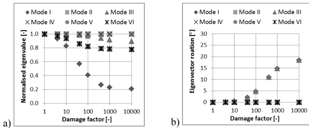
Fig. 6. Fibre damage effects: a) eigenvalue reduction, b) eigenvector roation.
