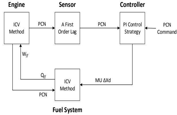
Fig. 7 Schematic of Integrated Engine, Controller and Fuel System
