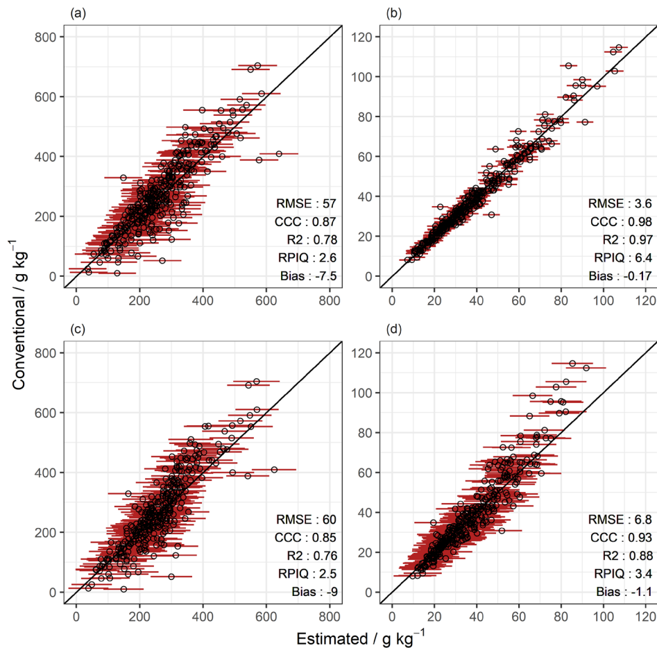
FIGURE 1 | Estimations of clay (a) and SOC (b) using partial least squares regression (PLSR) on a validation holdout set ( n=319 ) and (c) and (d) correspond to clay and SOC predictions by random forest (RF). Horizontal lines (–) are the total estimation error variances (Equation 2).
