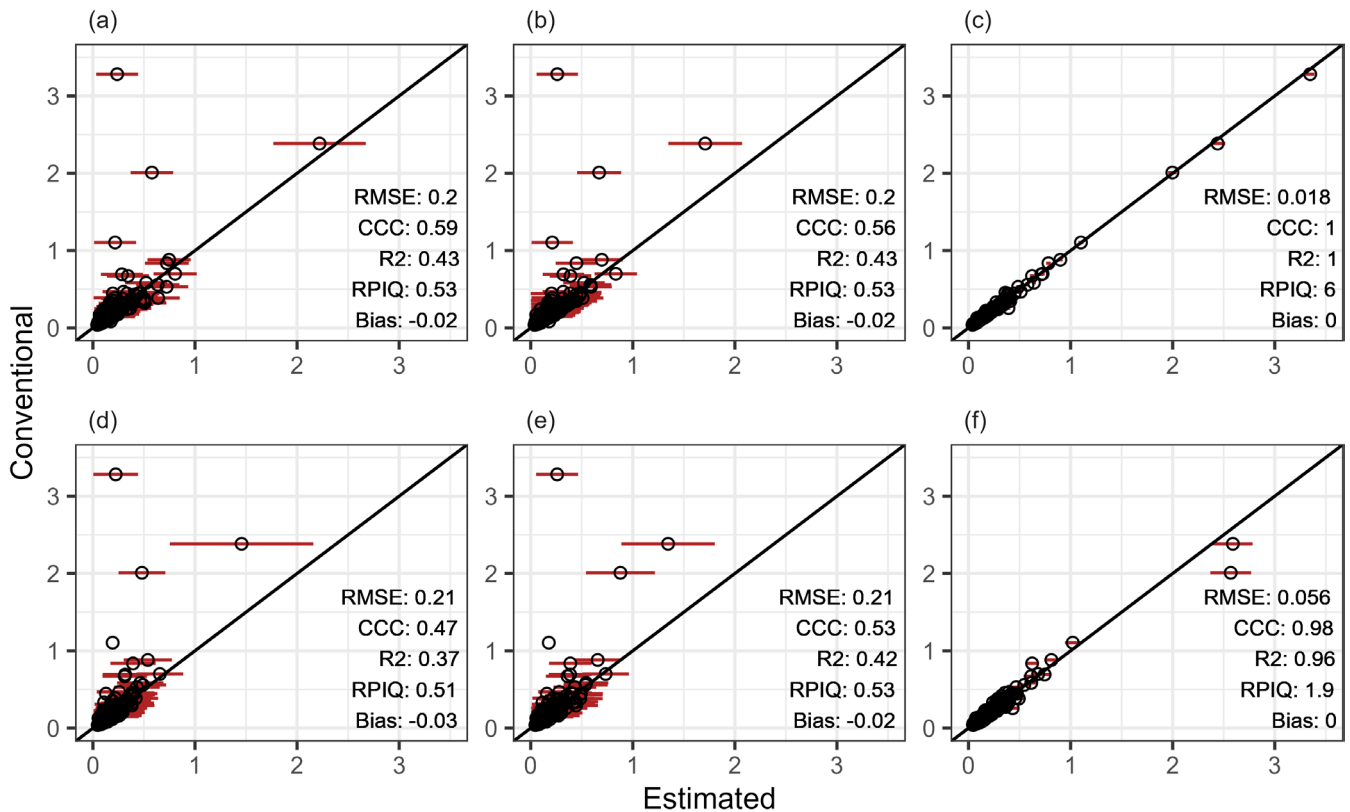
FIGURE 2 | Estimations of partial least squares regression (top-row) and random forest (bottom-row) on a validation holdout set ( n=319 ). Columns correspond to estimation methods: (\text{SOC}/\text{clay})_{\text{Est}} (a and d), \text{SOC}_{\text{Est}}/\text{clay}_{\text{Est}} (b and e) and \text{SOC}_{\text{Est}}/\text{clay}_{\text{Con}} (c and f). Horizontal bars (–) are the total estimation error variances (Equation 2).
