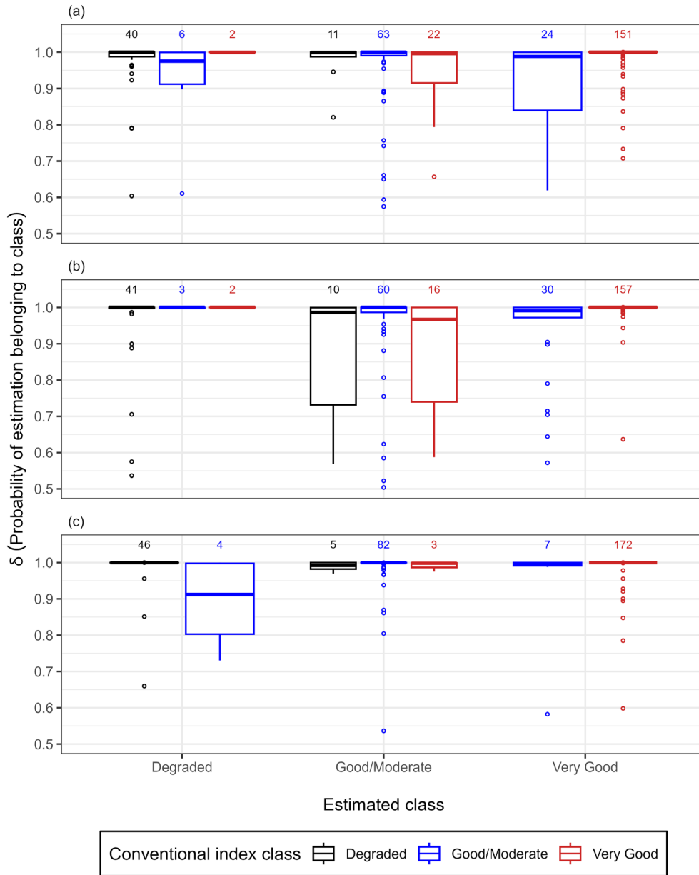
FIGURE 4 | Boxplots of the estimated index class probability ( \delta , Equation 3) as a function of the estimated index class, by different estimation method: (SOC/clay) Est (a); SOC Est /clay Est (b) and SOC Est /clay Con (c). Boxplots have been grouped and coloured by the index class based on conventionally measured data, with the corresponding count displayed above.
