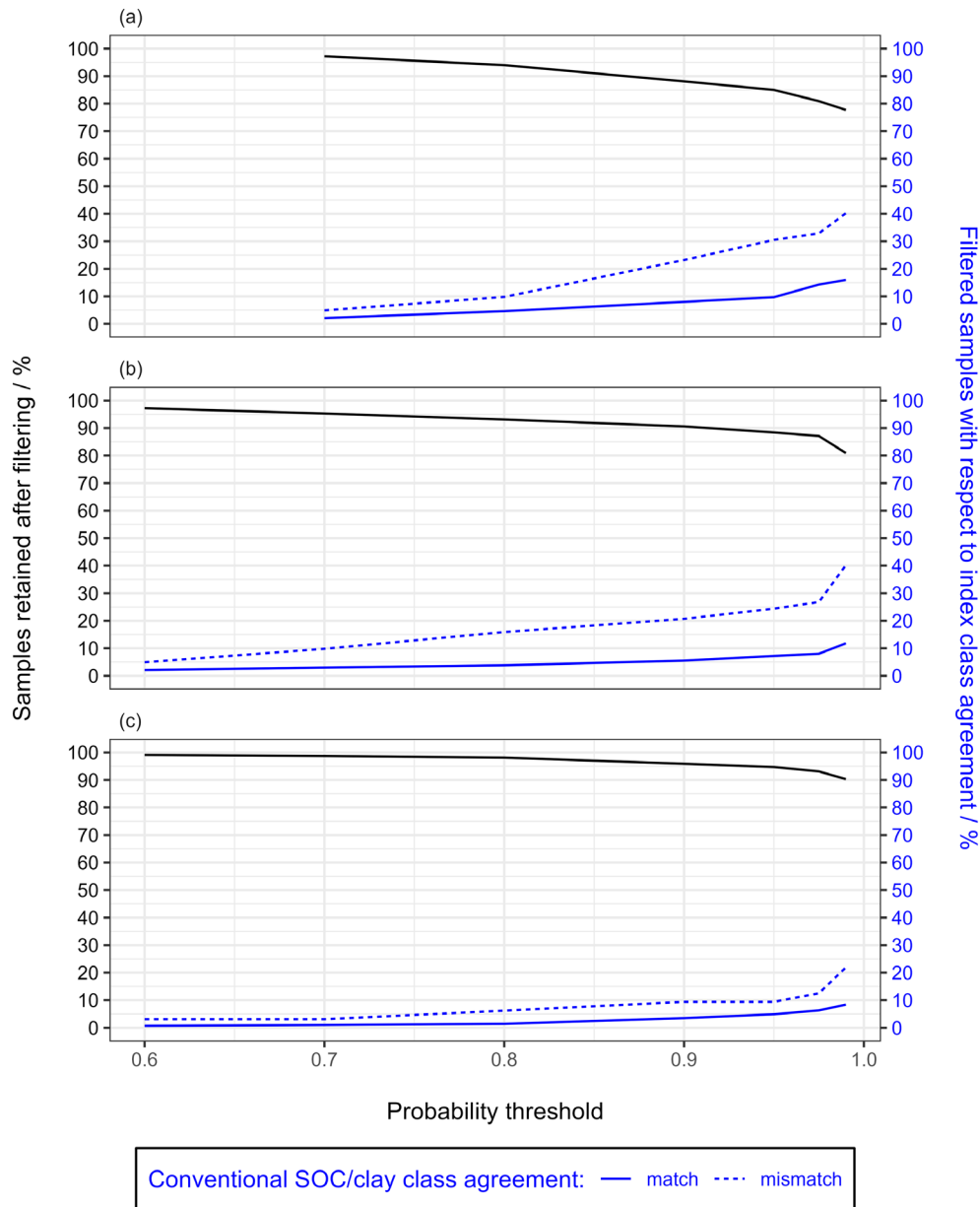
FIGURE 5 | Percentage of samples from the validation set retained after filtering based on the estimated SOC/clay class probability threshold (left y-axis, black line) and the filtered samples as a percentage of the number of samples with their respective index class agreement status (right y-axis, blue lines). Rows correspond to index estimation methods: (\text{SOC}/\text{clay})_{\text{Est}} (a), \text{SOC}_{\text{Est}}/\text{clay}_{\text{Est}} (b), and \text{SOC}_{\text{Est}}/\text{clay}_{\text{Con}} (c).
