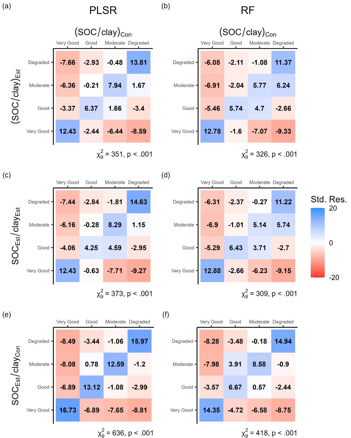
FIGURE 3 | Standardised residuals of chi-square tests for the validation set between conventional index class ((SOC/clay) Con , x-axis) and estimated index class (y-axis) for each of the estimation methods: (SOC/clay) Est (a and b), SOC Est /clay Est (c and d) and SOC Est /clay Con (e and f). The columns correspond to the regression methods: partial least squares regression (PLSR) and random forest (RF). Positive values suggest association of estimated and conventional classes; negative values suggest a lack of association.
