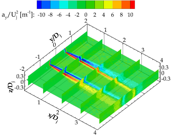
Figure 10: M 0.506 jet flow with streamwise slice at z/D_j = 0 and cross-stream slices at x/D_j = 0.2, 1, 2, 3, 4 . Top: normalised mean axial acceleration ( a_x/U_j^2 ). Bottom: normalised mean lateral acceleration ( a_y/U_j^2 ).
