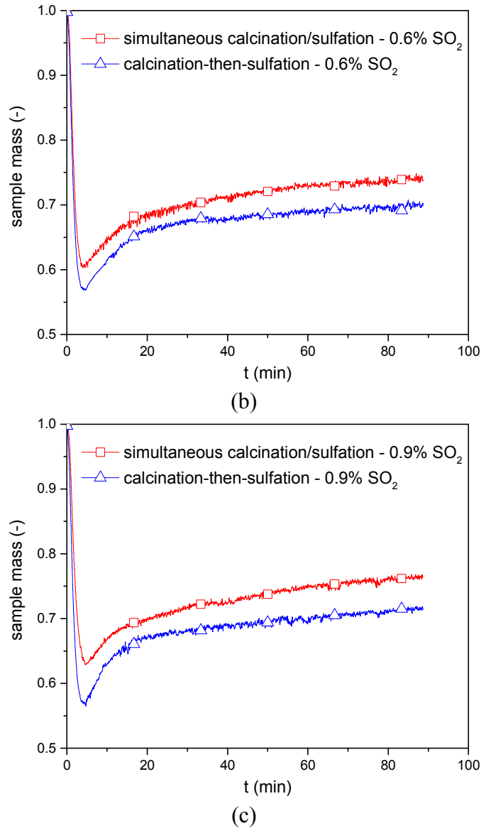
Fig. 2. Sample mass in simultaneous reaction and sequential reaction under different \text{SO}_2 concentrations. (a) 0.3% \text{SO}_2 ; (b) 0.6% \text{SO}_2 ; and (c) 0.9% \text{SO}_2 .
