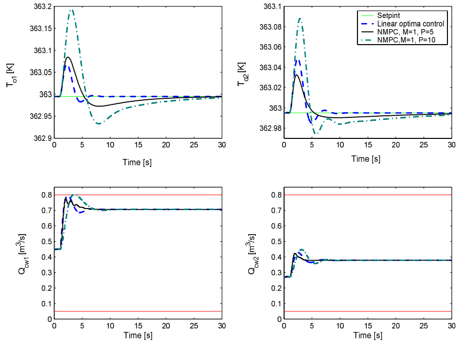
Figure 11: Two-CSTR performance during unmeasured disturbance rejection test ( -10 \text{ [K]} step change in T_{cw1} and T_{cw2} at t = 2 \text{ [s]} ).
