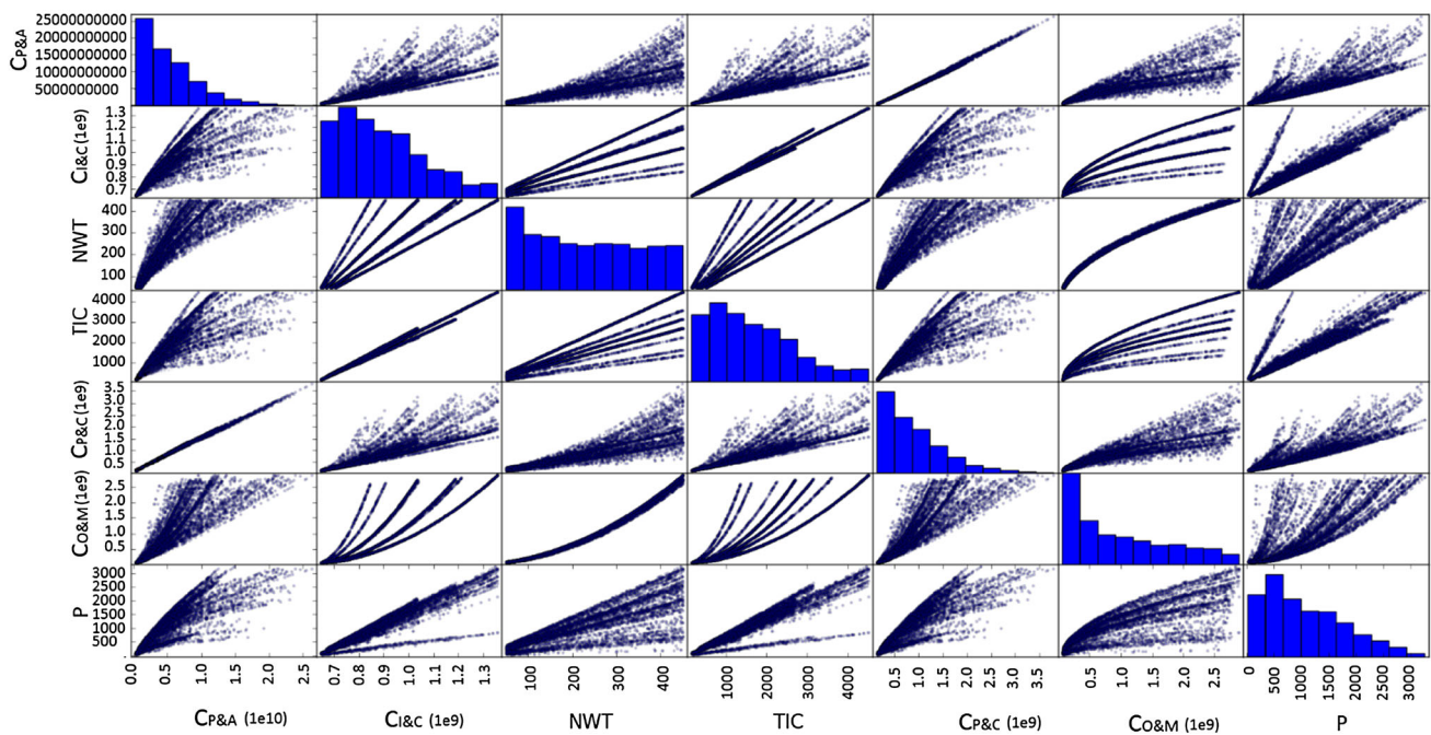
Fig. 8 Scatter plot matrix among the seven objectives, i.e., C_{P\&A} , C_{P\&C} , C_{I\&C} , C_{O\&M} , NWT, P, and TIC using NSGAIII
