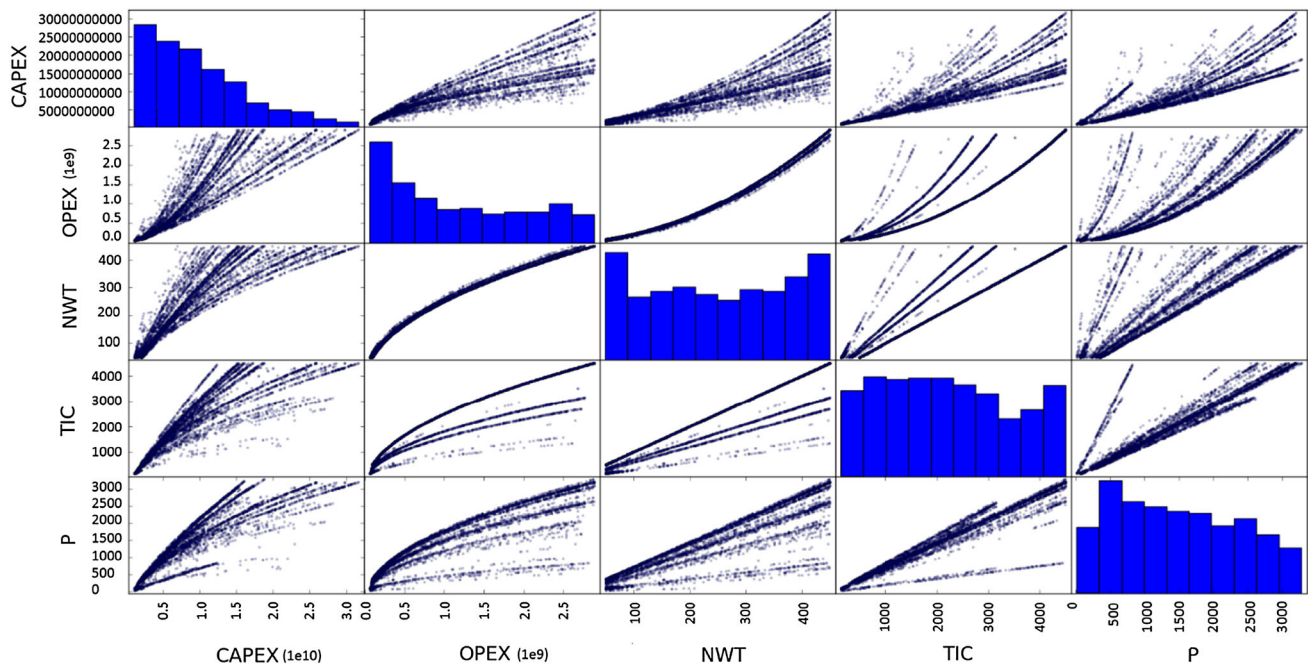
Fig. 7 Scatter plot matrix among CAPEX, OPEX, NWT, P, and TIC using NSGAII
