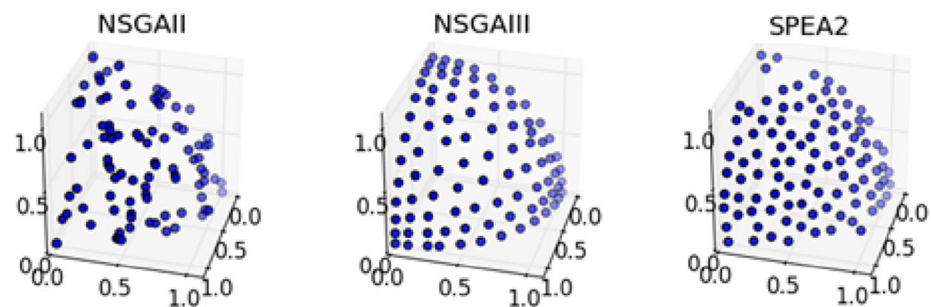
Fig. 2 NSGA II, III and SPEA2 ( Hadka 2015 ) demonstrating the distribution of solutions when applied to a benchmark function with three objectives
