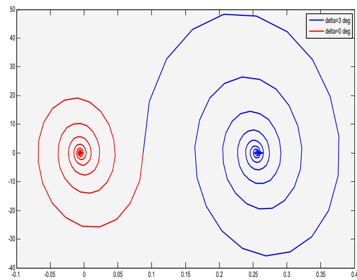
Figure 28. The state space response of \beta without freeplay and with 2^\circ freeplay. (In flutter speed).
