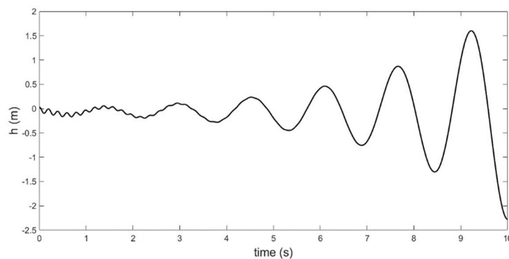
Figure 13. Time response of “h” in upper speed of flutter (35 m/s).
