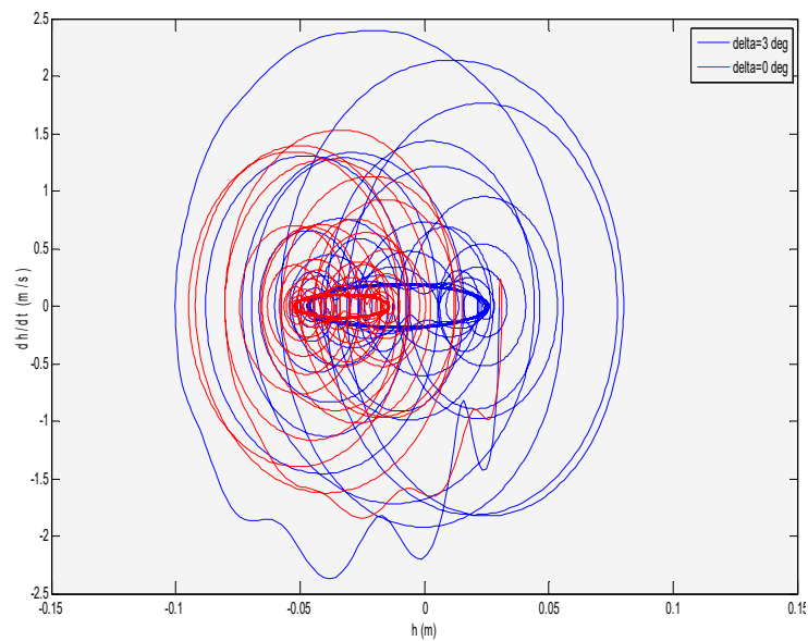
Figure 29. The state space response of “h” without freeplay and with 2^\circ freeplay. (In flutter speed).
