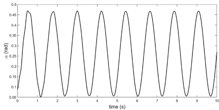
Figure 8. Time response of alpha in flutter speed (23.9 m/s).
