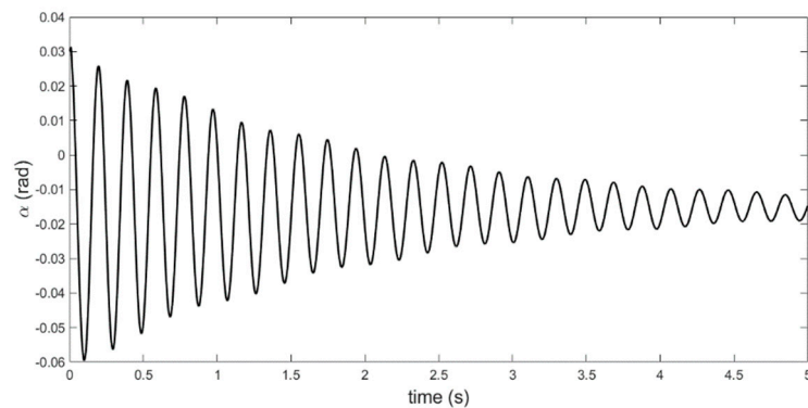
Figure 5. Time response of alpha in lower speed of flutter (20 m/s).
