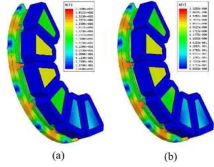
Fig. 3. Open-circuit flux density distributions at 7-axis rotor position. (a) Isotropic model. (b) Anisotropic model.
