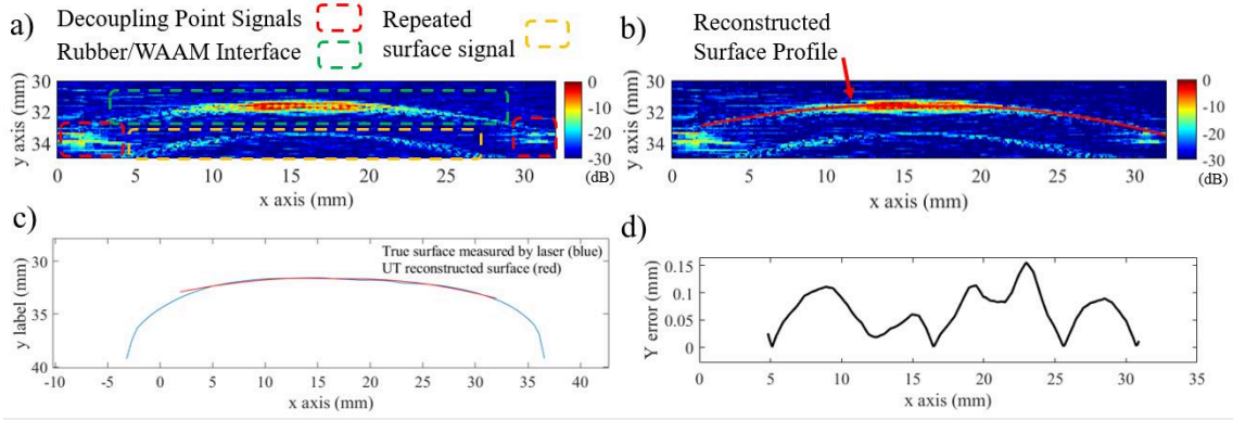
Figure 10 (a) An image of the WAAM surface formed using the dual-medium SAFT algorithm, (b) fitted curve to the extracted high-intensity surface points of the SAFT image after filtering and denoising, (c) comparison between the laser-scanned surface profile and the SAFT reconstructed profile, and (d) measured error between the surface profile acquired by laser and through SAFT reconstruction of the Ti-64 WAAM with bottom-drilled holes
