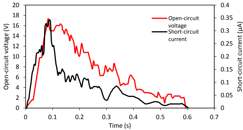
Figure 12: Open-circuit voltage V_{oc} and short-circuit current I_{sc} when applying bending force at 1 Hz on the 0.2 wt% Ag + CIP composite
