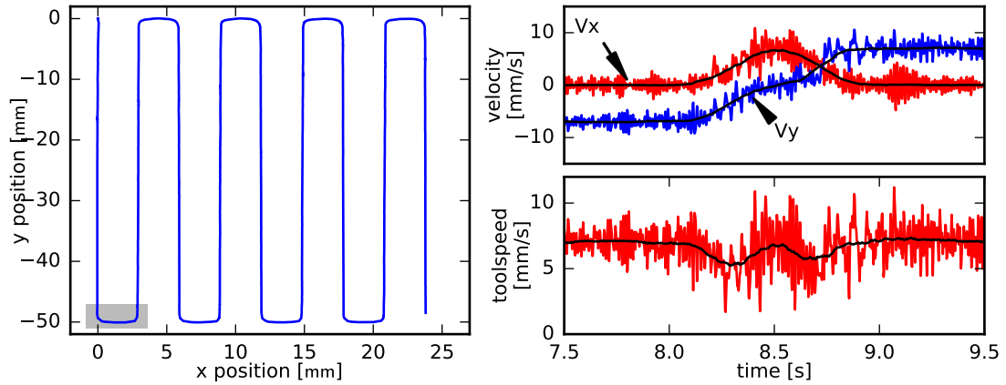
Figure 7. a) Oscillatory wall building path; arrows show direction of travel and highlighted rectangle showing the path traversed in a). b) Velocity and tool speed vs time.
